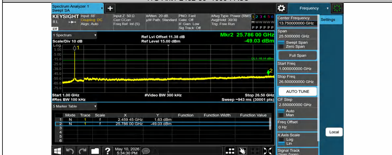
11G-Ant1-2462-1000~26500-PASS
