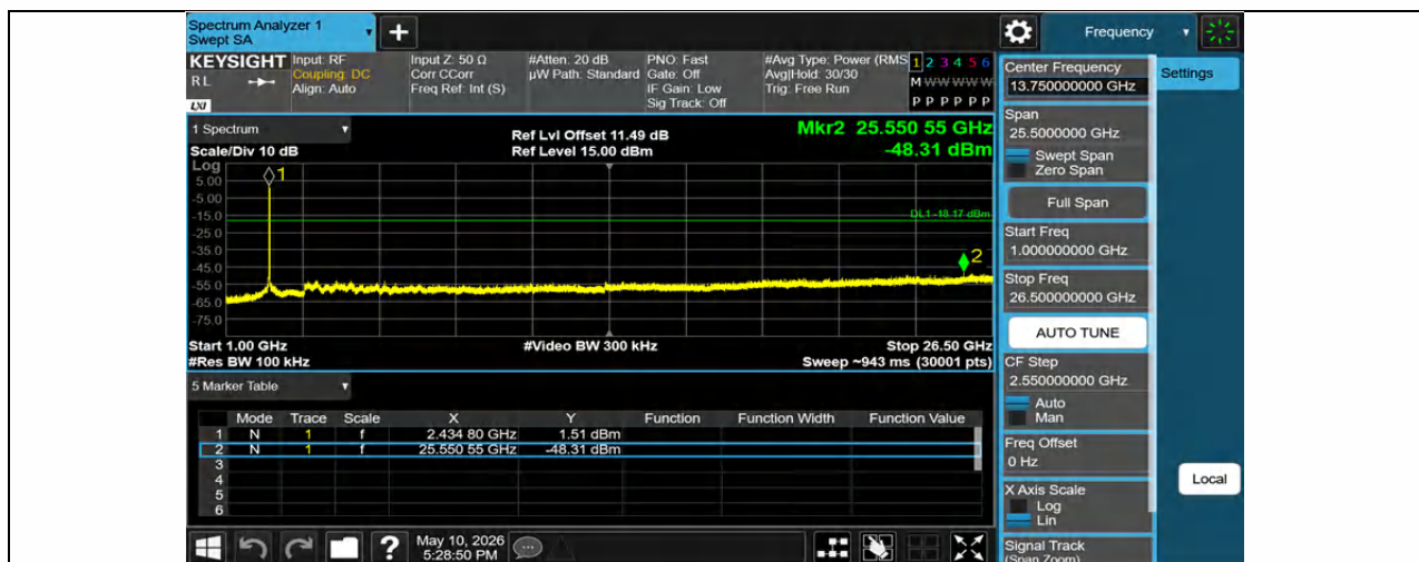
11G-Ant1-2437-1000~26500-PASS
