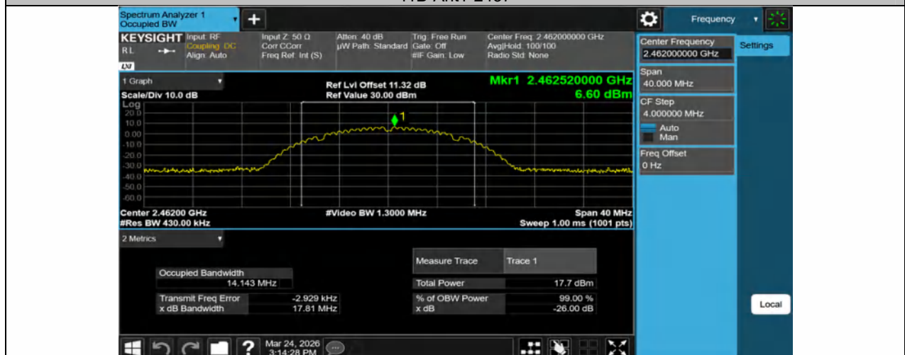
11B-Ant1-2462
