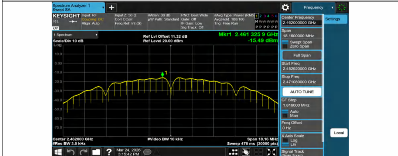
11B-Ant1-2462-PASS
