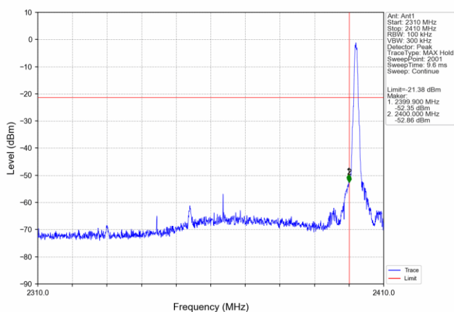
1M_LCH_2402MHz_Ant1_NTNV
