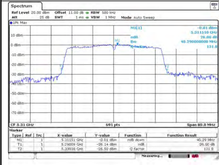
26dB Bandwidth
