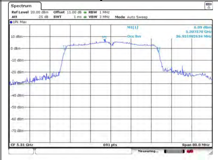
99% Occupied Bandwidth
