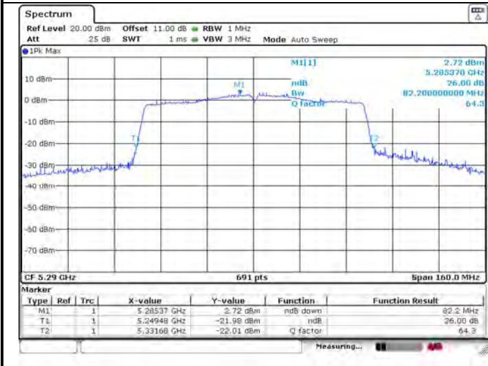
26dB Bandwidth
