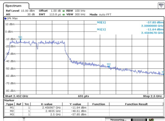
CH11-Bandedge
