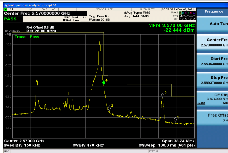
Band7-15MHz-16QAM-21375-1RB#74
