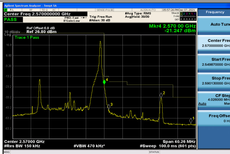
Band7-15MHz-QPSK-21375-1RB#74
