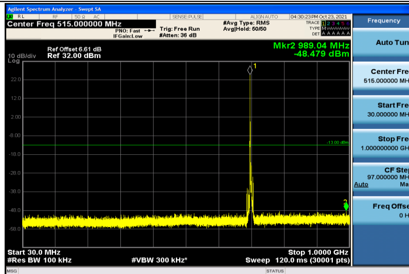
Band17-5MHz-16QAM-23755-1RB#0-30~1000MHz
