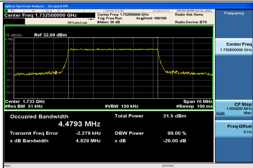
Band4-5MHz-QPSK-20175-25RB#0-4.4793
