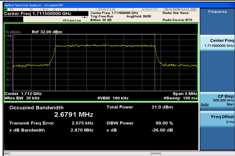
Band4-3MHz-QPSK-19965-15RB#0-2.6791
