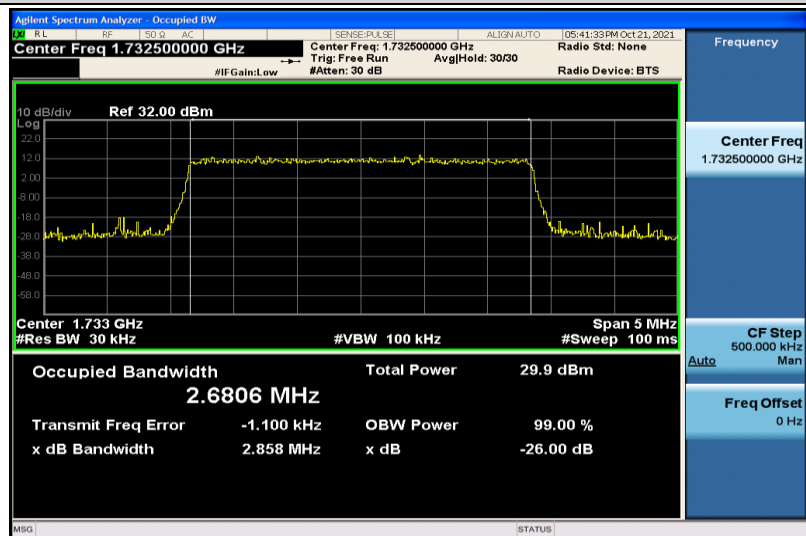
Band4-3MHz-16QAM-20175-15RB#0-2.6806
