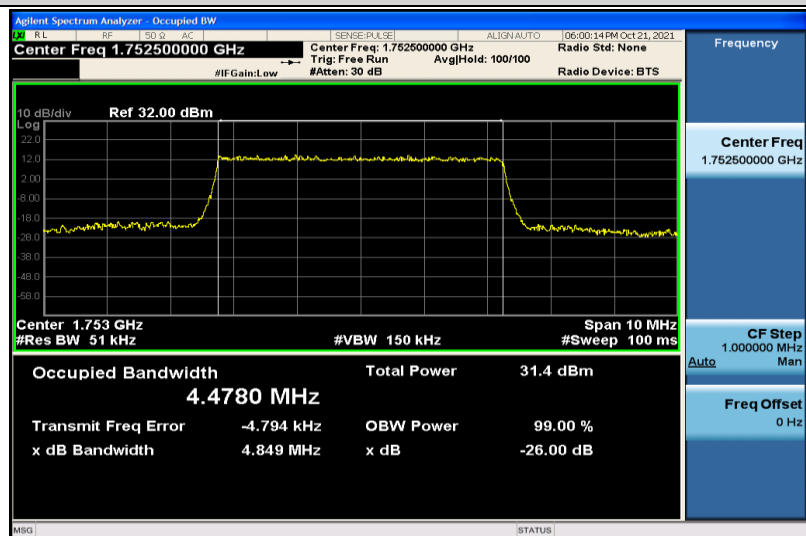
Band4-5MHz-QPSK-20375-25RB#0-4.4780
