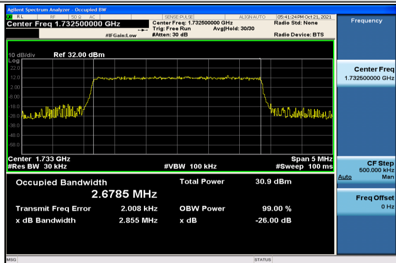
Band4-3MHz-QPSK-20175-15RB#0-2.6785
