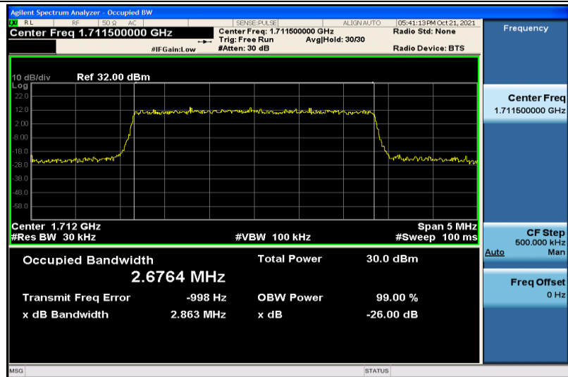
Band4-3MHz-16QAM-19965-15RB#0-2.6764
