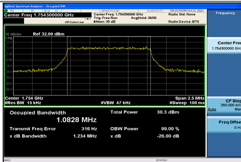
Band4-1.4MHz-QPSK-20393-6RB#0-1.0828
