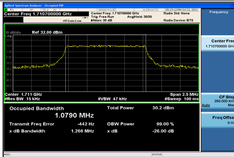
Band4-1.4MHz-QPSK-19957-6RB#0-1.0790
