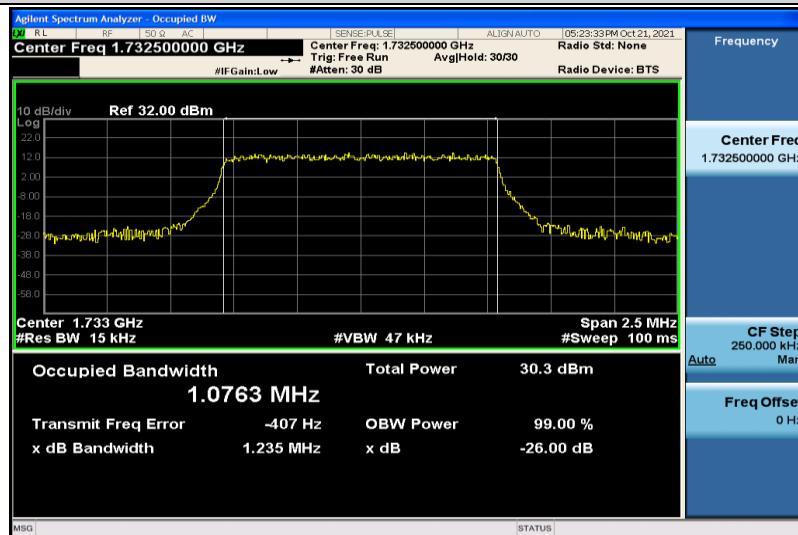
Band4-1.4MHz-QPSK-20175-6RB#0-1.0763
