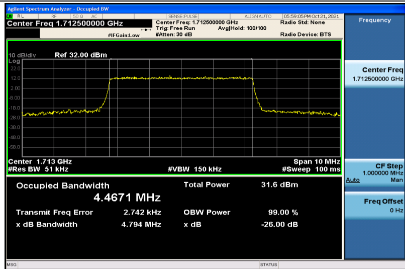
Band4-5MHz-QPSK-19975-25RB#0-4.4671
