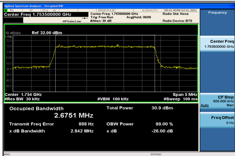
Band4-3MHz-QPSK-20385-15RB#0-2.6751
