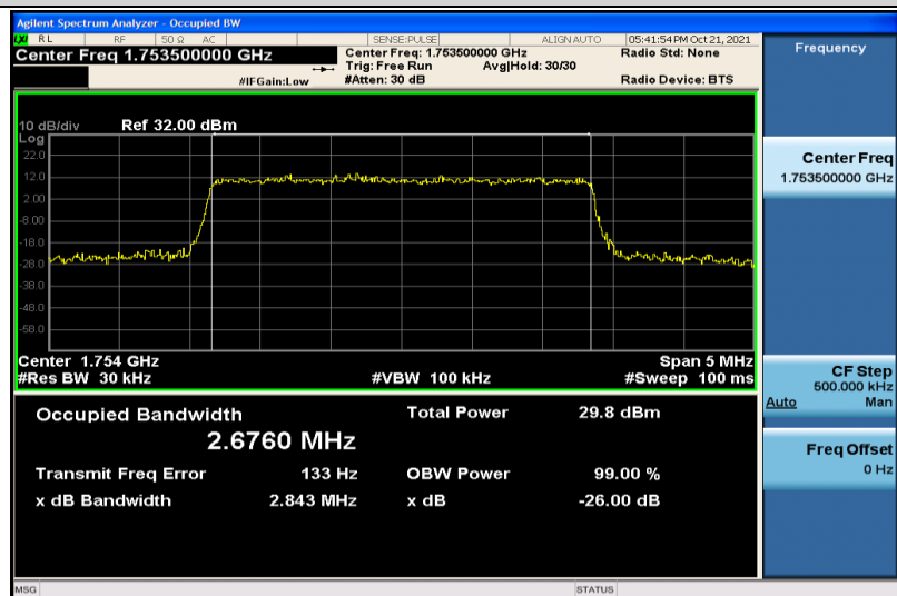
Band4-3MHz-16QAM-20385-15RB#0-2.6760
