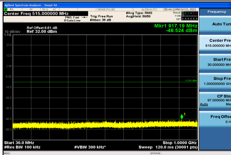
Band4-3MHz-16QAM-19965-1RB#0-30~1000MHz
