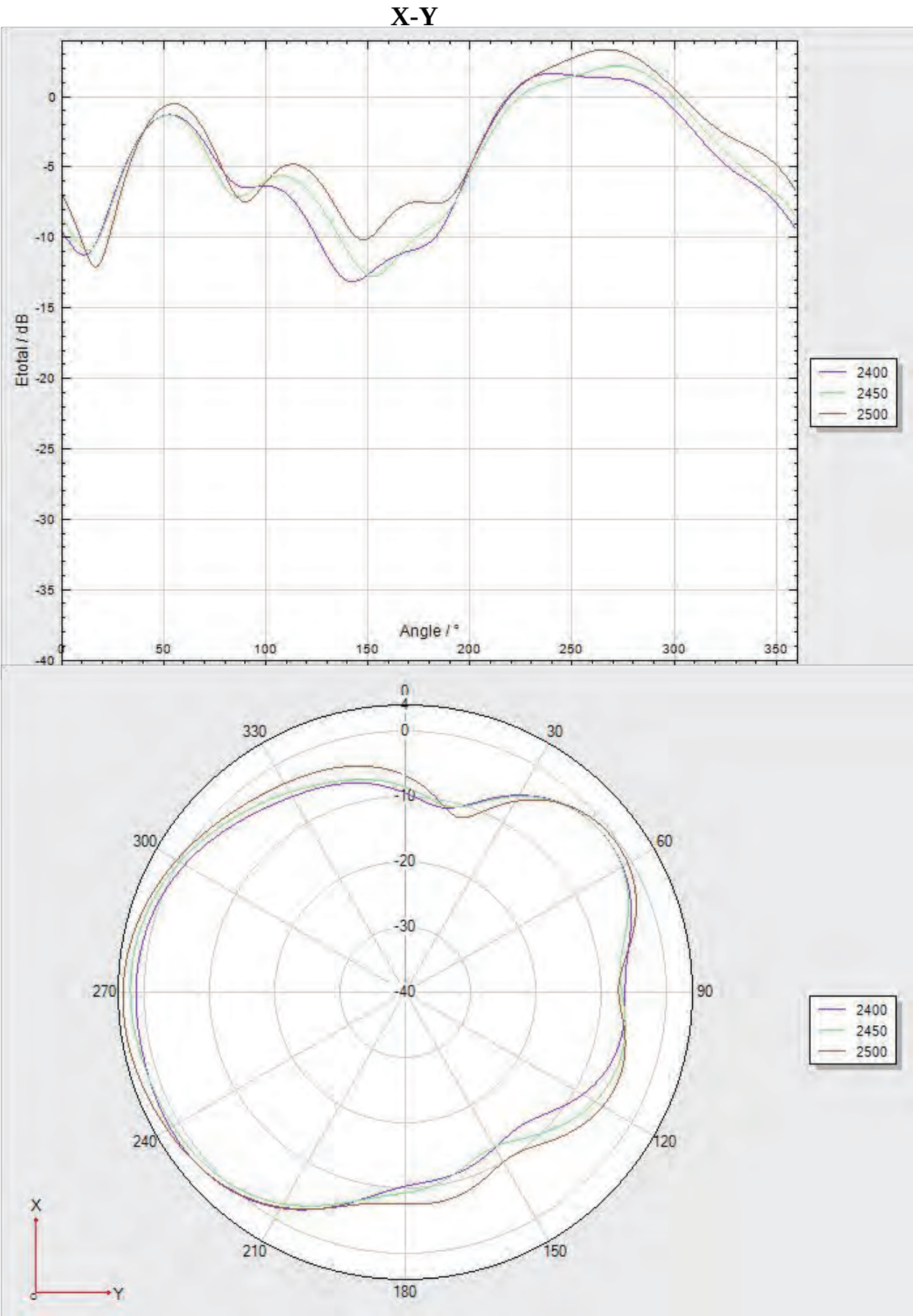
Theta 90 2D figure
