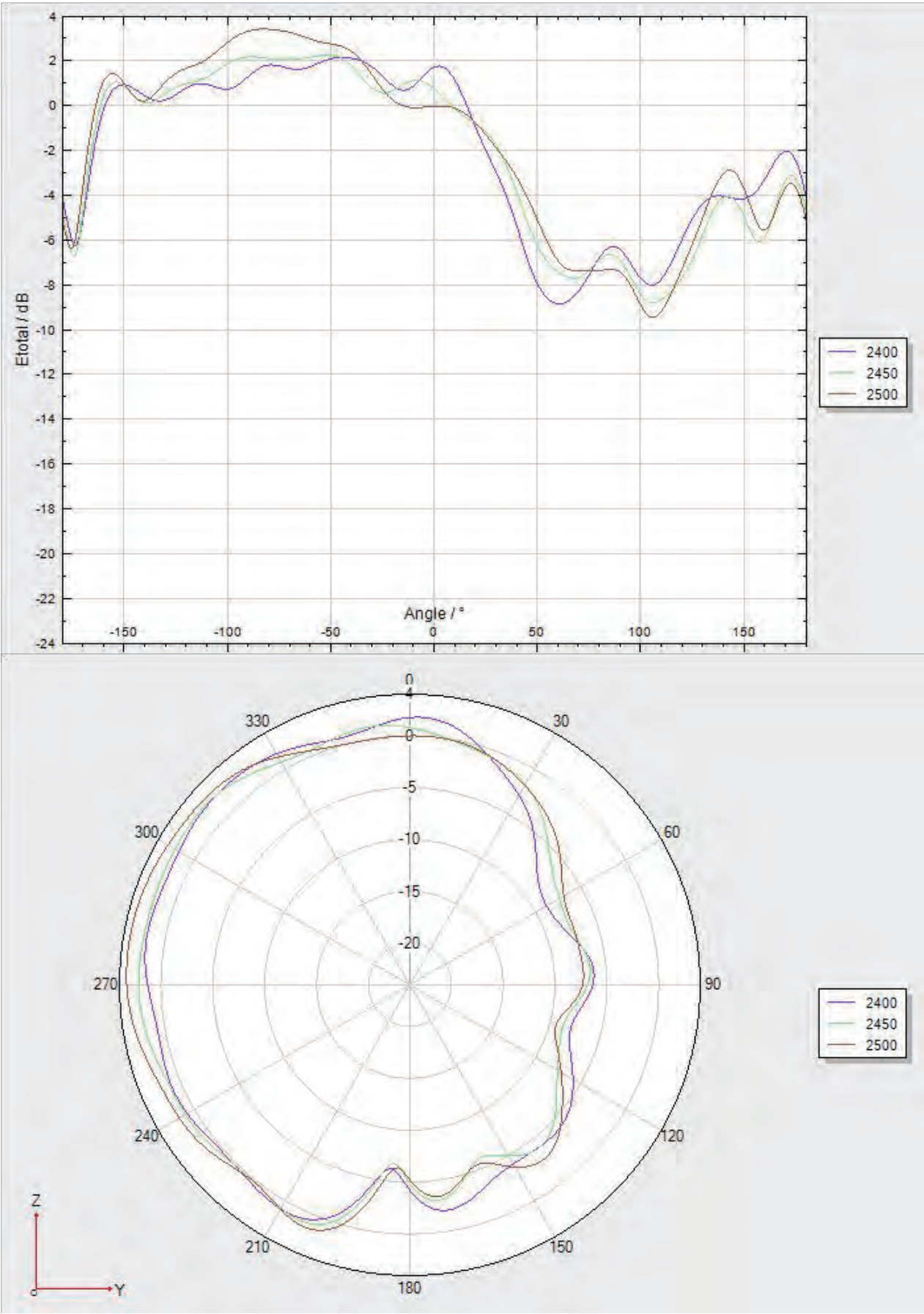
Phi 90 2D figure
