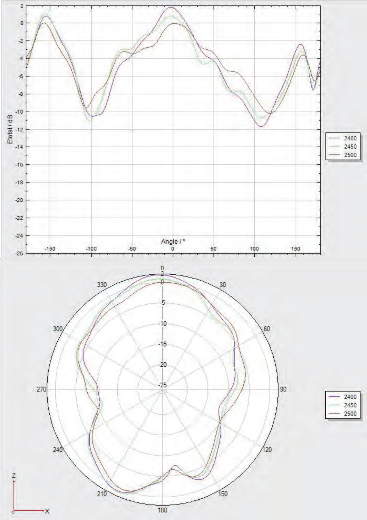
Phi 0 2D figure X-Z
