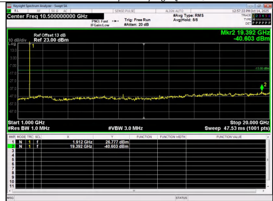
1000.0MHz-20000.0MHz Band 2 3MHz/1908.5/High 16QAM 1@0
