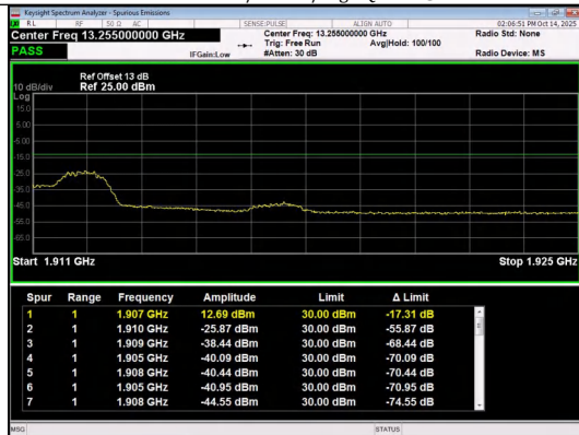
Band 2 3MHz/1908.5/High 16QAM 1@0
