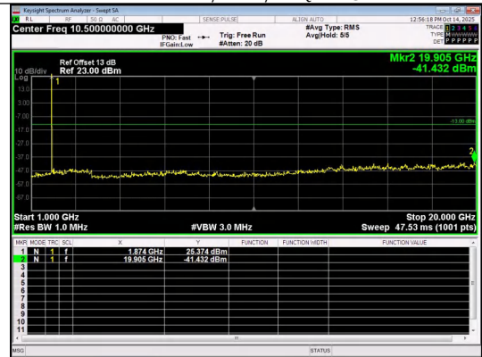
1000.0MHz-20000.0MHz Band 2 3MHz/1880.0/Mid 16QAM 1@0
