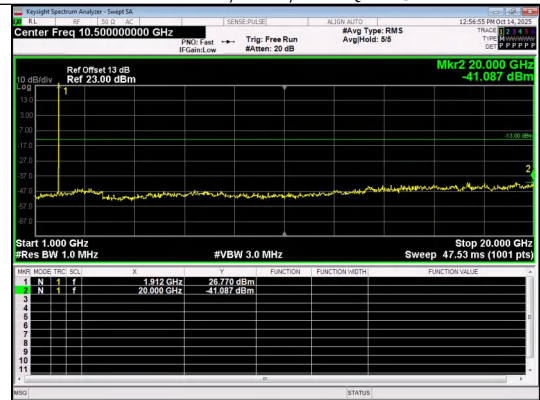
1000.0MHz-20000.0MHz Band 2 3MHz/1908.5/High QPSK 1@0
