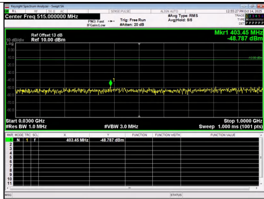
30.0MHz-1000.0MHz Band 2 3MHz/1880.0/Mid QPSK 1@0
