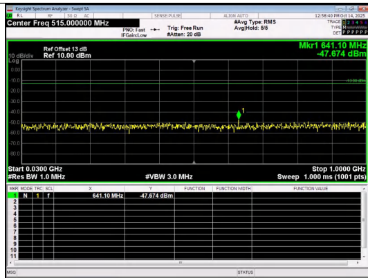
30.0MHz-1000.0MHz Band 2 5MHz/1852.5/Low QPSK 1@0
