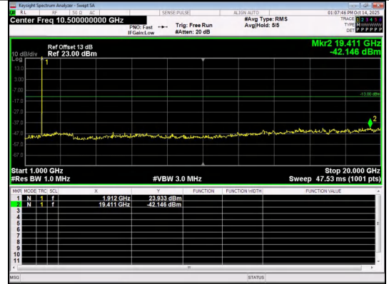
1000.0MHz-20000.0MHz Band 2 5MHz/1907.5/High 16QAM 1@0
