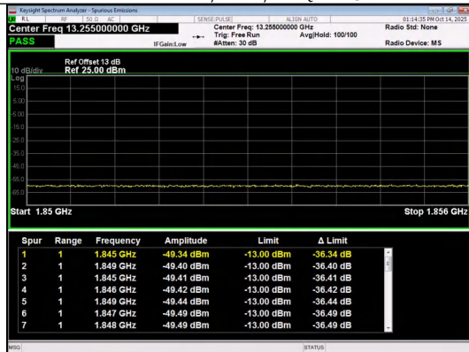
Band 2 1.4MHz/1850.7/Low 16QAM 1@5
