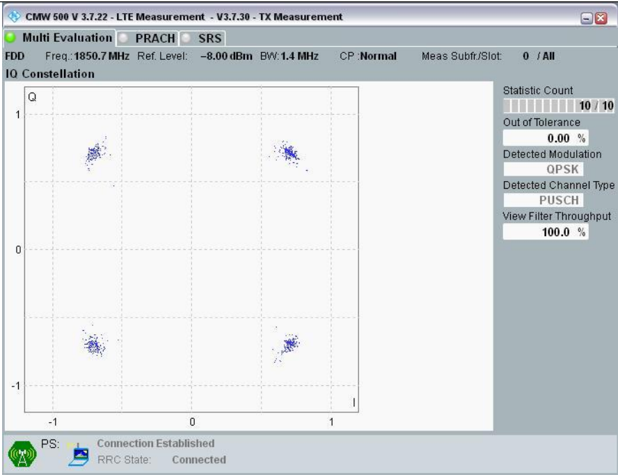
CMW_65_NT_NV_0_Band_2_QPSK_1_4M_CH18607_6_0
