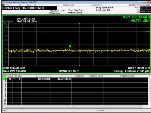
30.0MHz-1000.0MHz Band 2 5MHz/1907.5/High 16QAM 1@0
