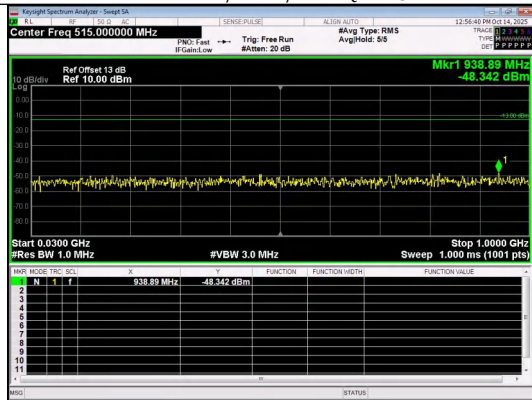
30.0MHz-1000.0MHz Band 2 3MHz/1908.5/High QPSK 1@0
