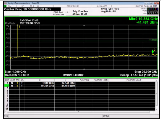
1000.0MHz-20000.0MHz Band 2 5MHz/1907.5/High QPSK 1@0
