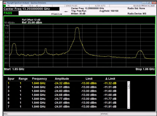
Band 2 5MHz/1852.5/Low 16QAM 1@24
