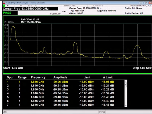
Band 2 5MHz/1852.5/Low 16QAM 1@0
