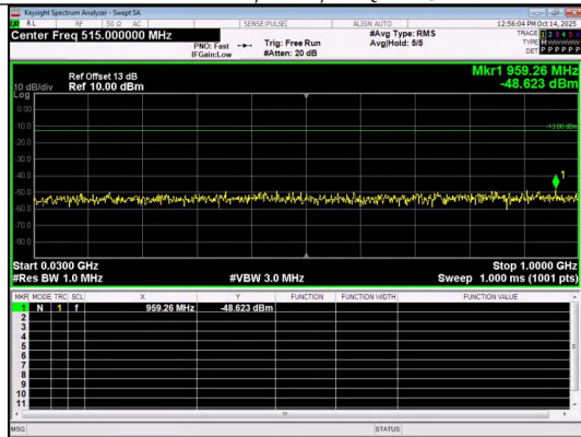
30.0MHz-1000.0MHz Band 2 3MHz/1880.0/Mid 16QAM 1@0
