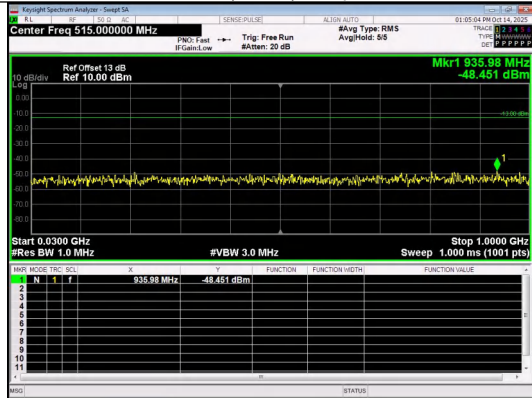
30.0MHz-1000.0MHz Band 2 5MHz/1852.5/Low 16QAM 1@0
