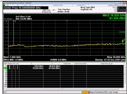
1000.0MHz-20000.0MHz Band 2 3MHz/1880.0/Mid QPSK 1@0
