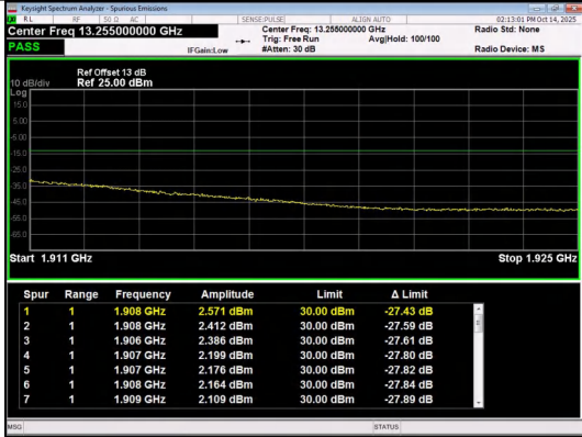
Band 2 5MHz/1907.5/High 16QAM 25@0
