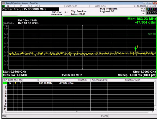
30.0MHz-1000.0MHz Band 2 5MHz/1907.5/High QPSK 1@0
