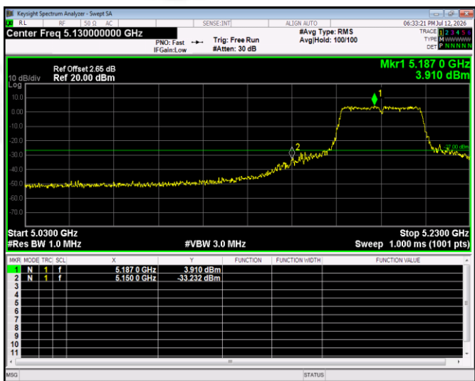
(802.11ac80) Band Edge - Channel 42
