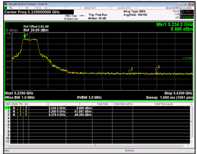
(802.11n20) Band Edge, Right Side
