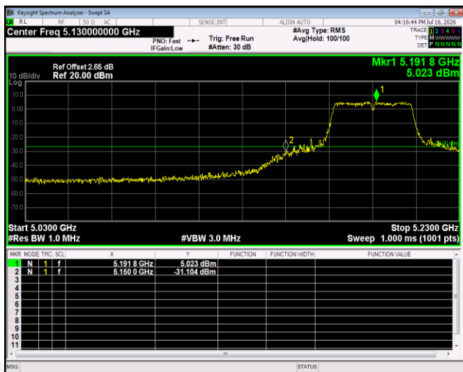
(802.11n40) Band Edge, Left Side
