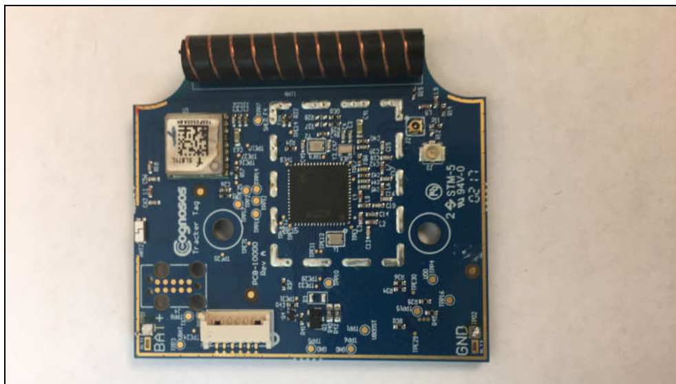
Figure 2: Internal Photo
