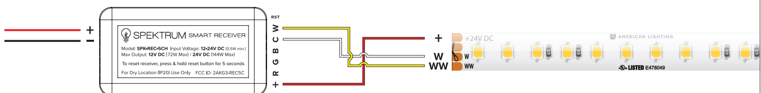
FIGURE 3 - Tunable CCT (3-Wire) Wiring Diagram
