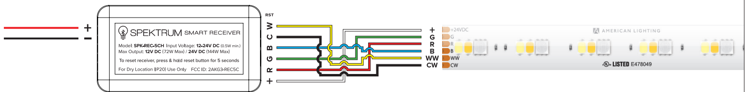
FIGURE 6 - RGB+TW (6-Wire) Wiring Diagram
