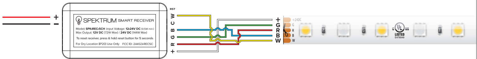
FIGURE 5 - RGBW (5-Wire) Wiring Diagram
