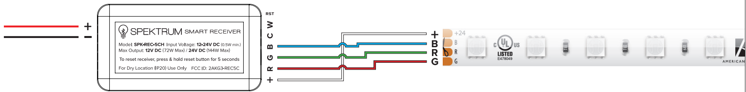
FIGURE 4 - RGB (4-Wire) Wiring Diagram
