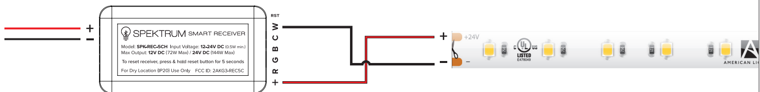
FIGURE 2 - Single Color (2-Wire) Wiring Diagram
