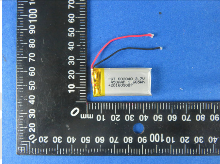
6. Figure The EUT-Battery View
