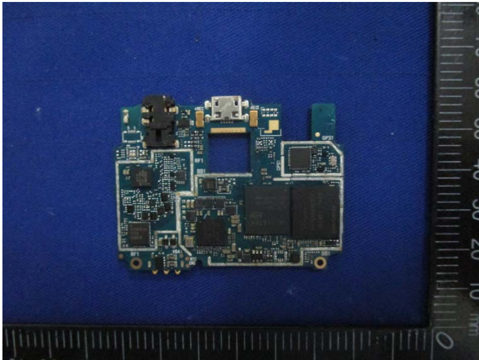
EUT – Main PCB Back Without Cover View
