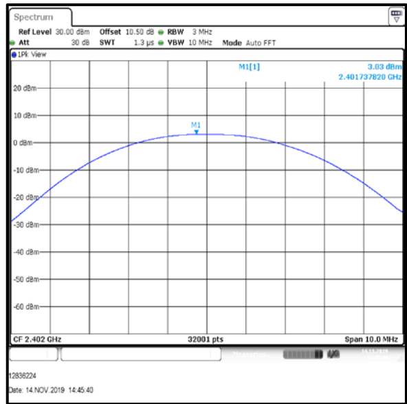
Bottom Channel
