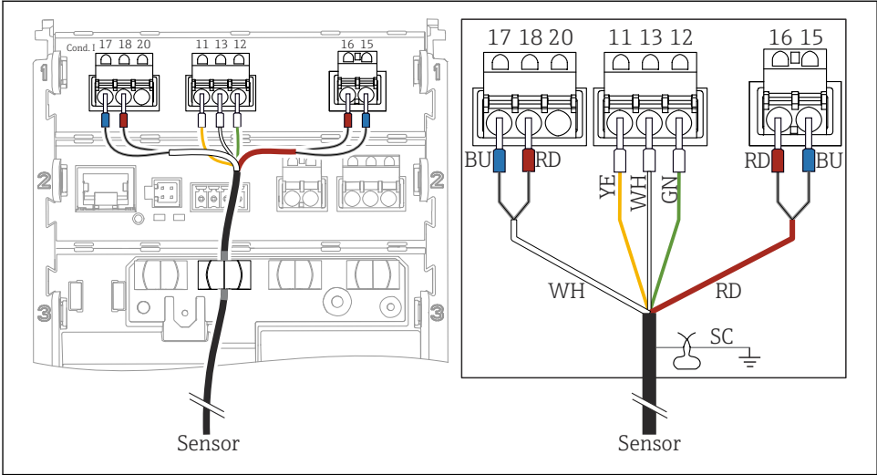
28 Device view
