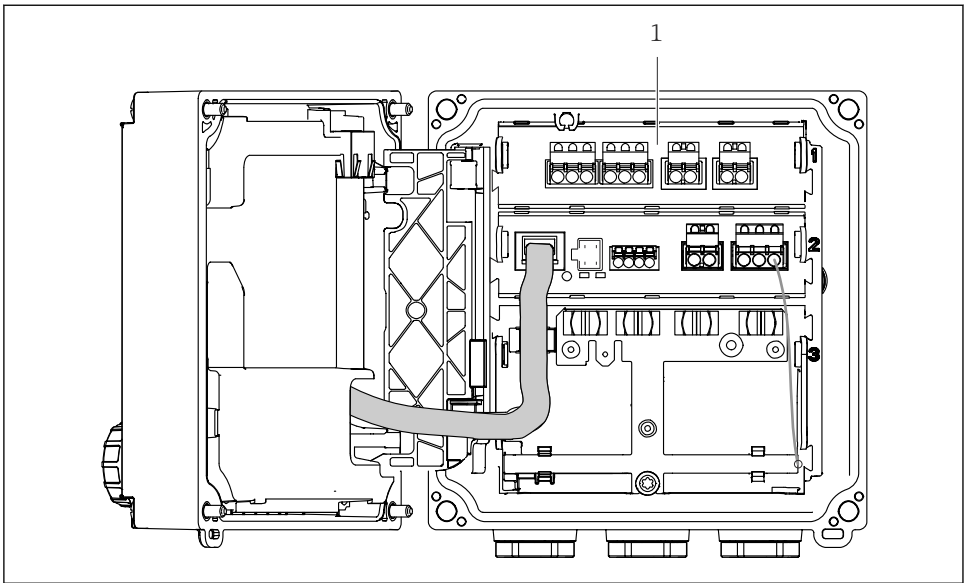
1 Connection area for analog sensors (different layout depending on the version)
