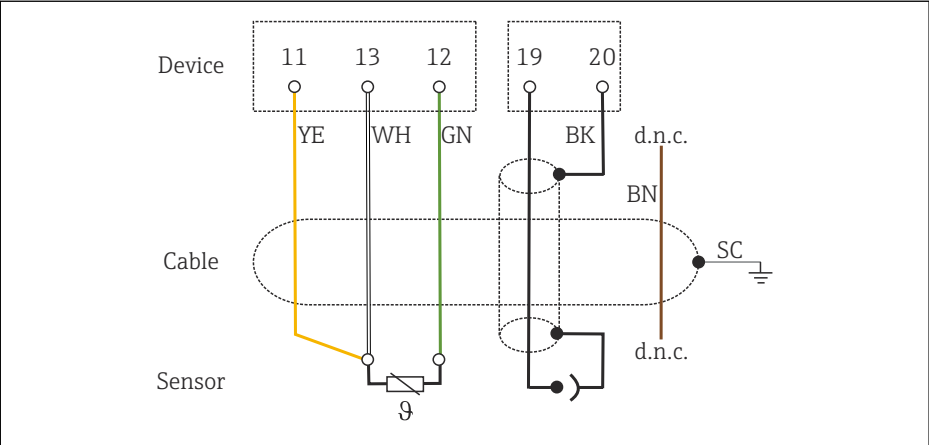
32 Wiring diagram
