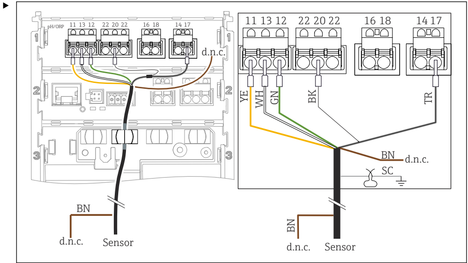
36 Device view
