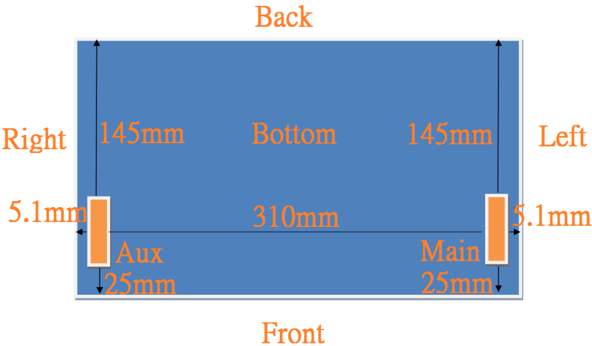
Figure of antenna location
