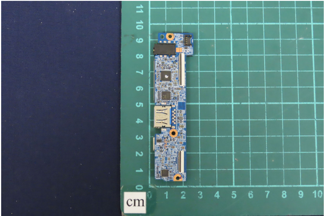
(22) EUT Photo
