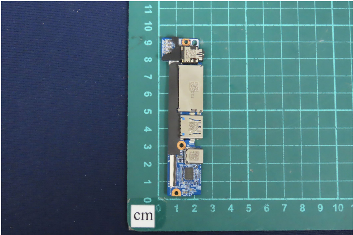
(23) EUT Photo
