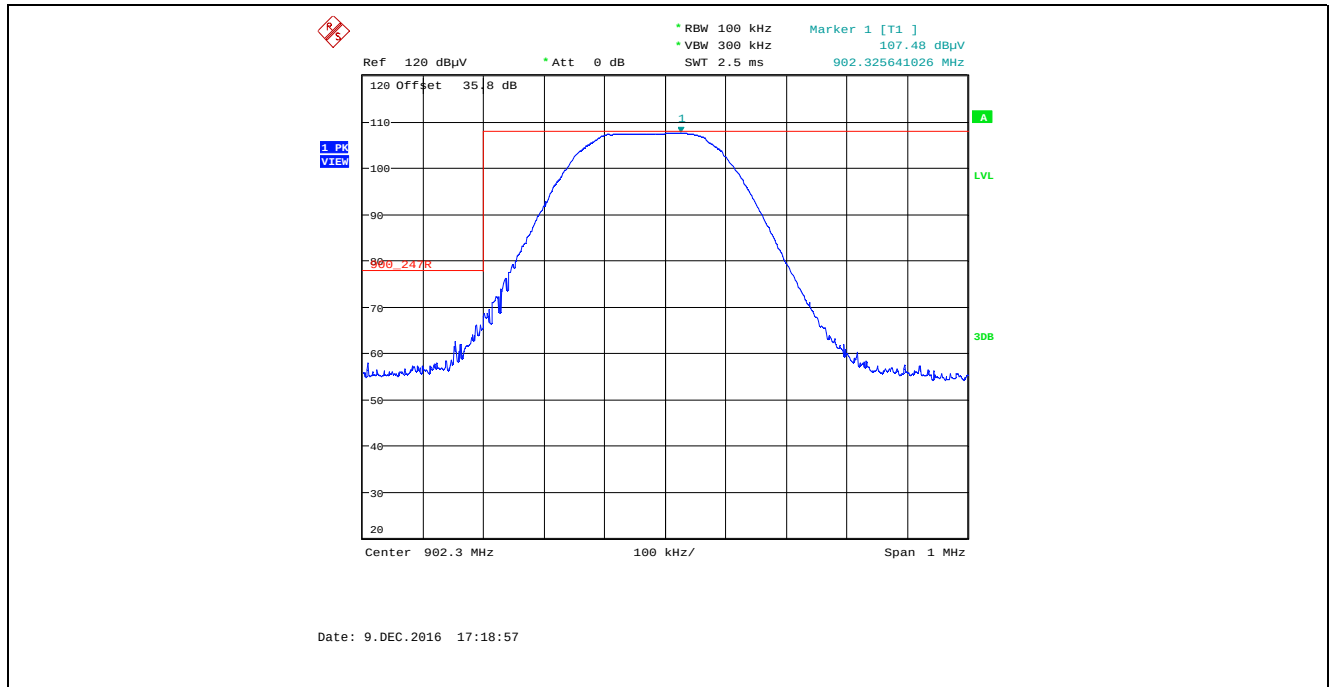
Plot 5.4.4.2.27. Band-Edge RF Radiated Emissions at 3 m, Vertical Polarization, 5470 bps Data Rate Single Frequency Mode, Low End of Frequency Band
