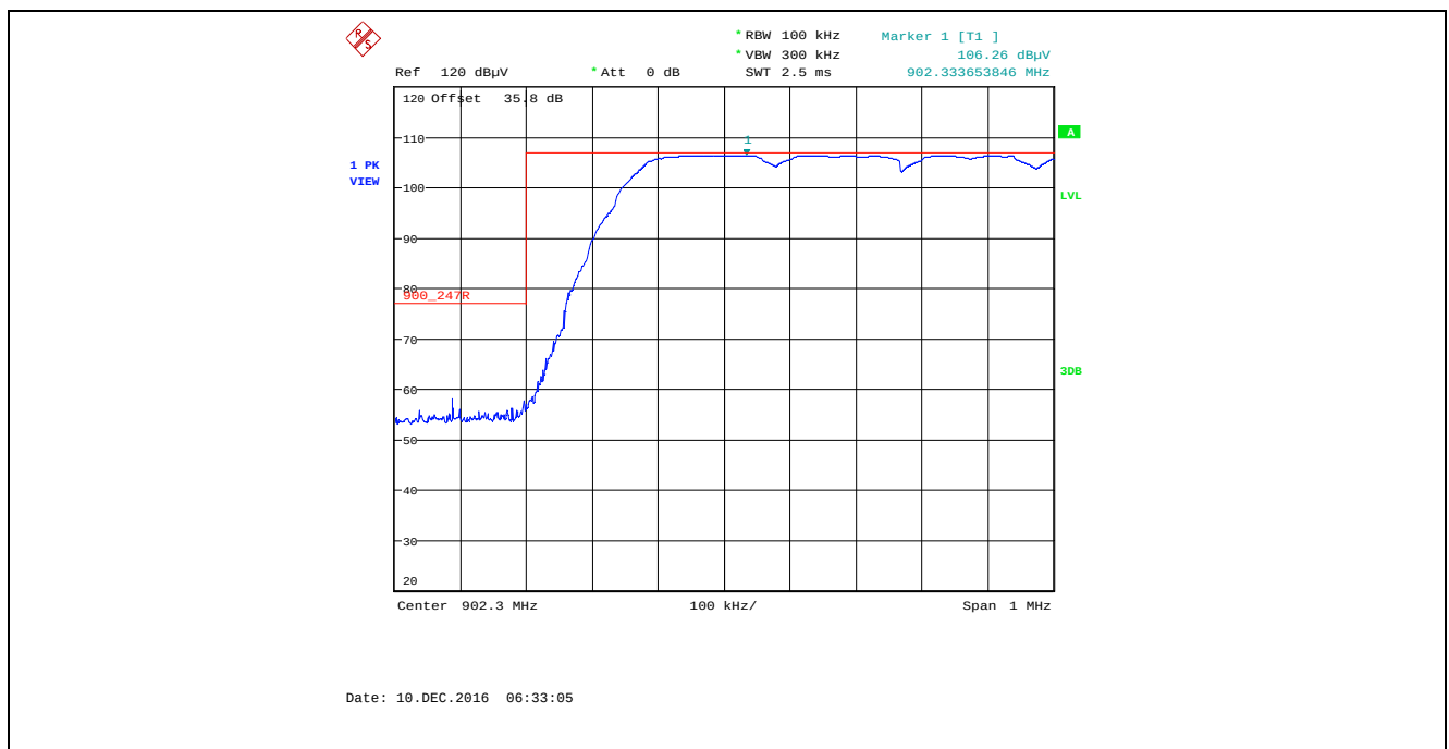
Plot 5.4.4.2.28. Band-Edge RF Radiated Emissions at 3 m, Vertical Polarization, 5470 bps Data Rate Pseudorandom Channel Hopping Mode, Low End of Frequency Band
