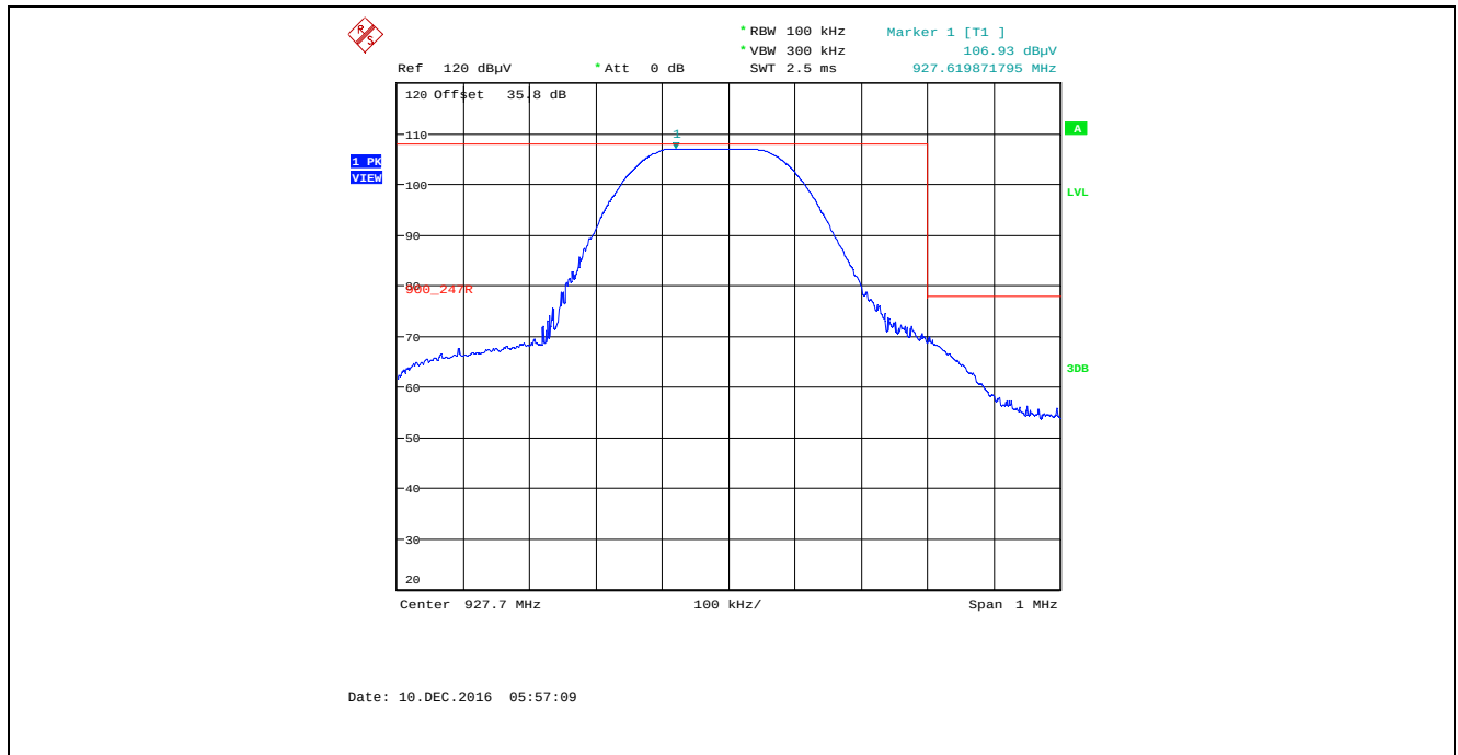
Plot 5.4.4.2.21. Band-Edge RF Radiated Emissions at 3 m, Horizontal Polarization, 3125 bps Data Rate Single Frequency Mode, High End of Frequency Band
