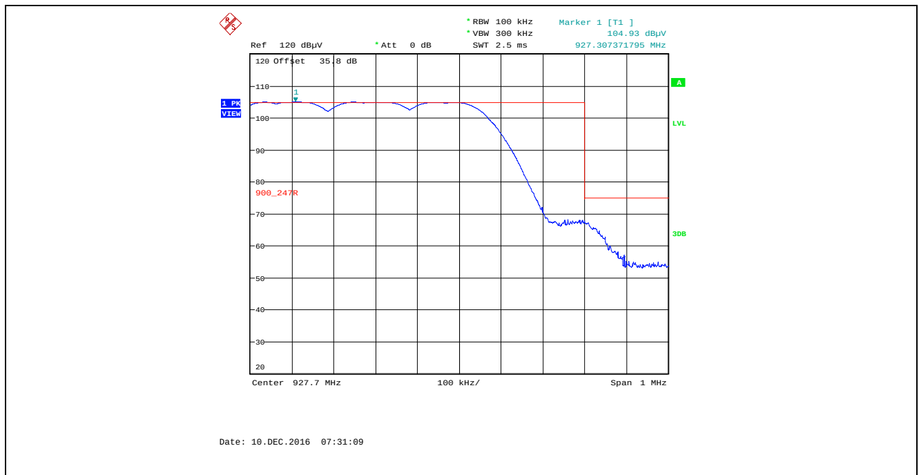
Plot 5.4.4.2.22. Band-Edge RF Radiated Emissions at 3 m, Horizontal Polarization, 3125 bps Data Rate Pseudorandom Channel Hopping Mode, High End of Frequency Band
