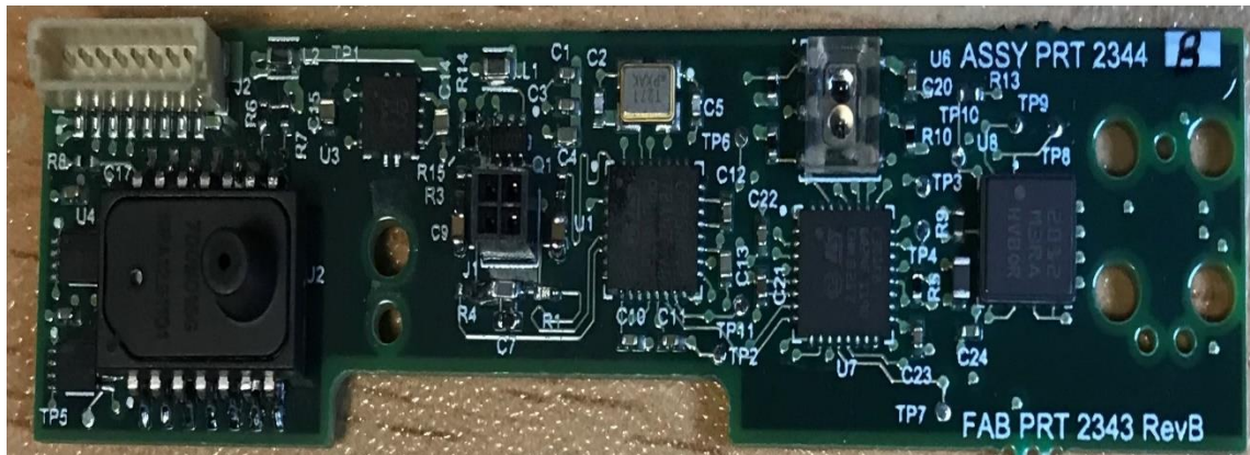
Figure 2: PCB Top Side
