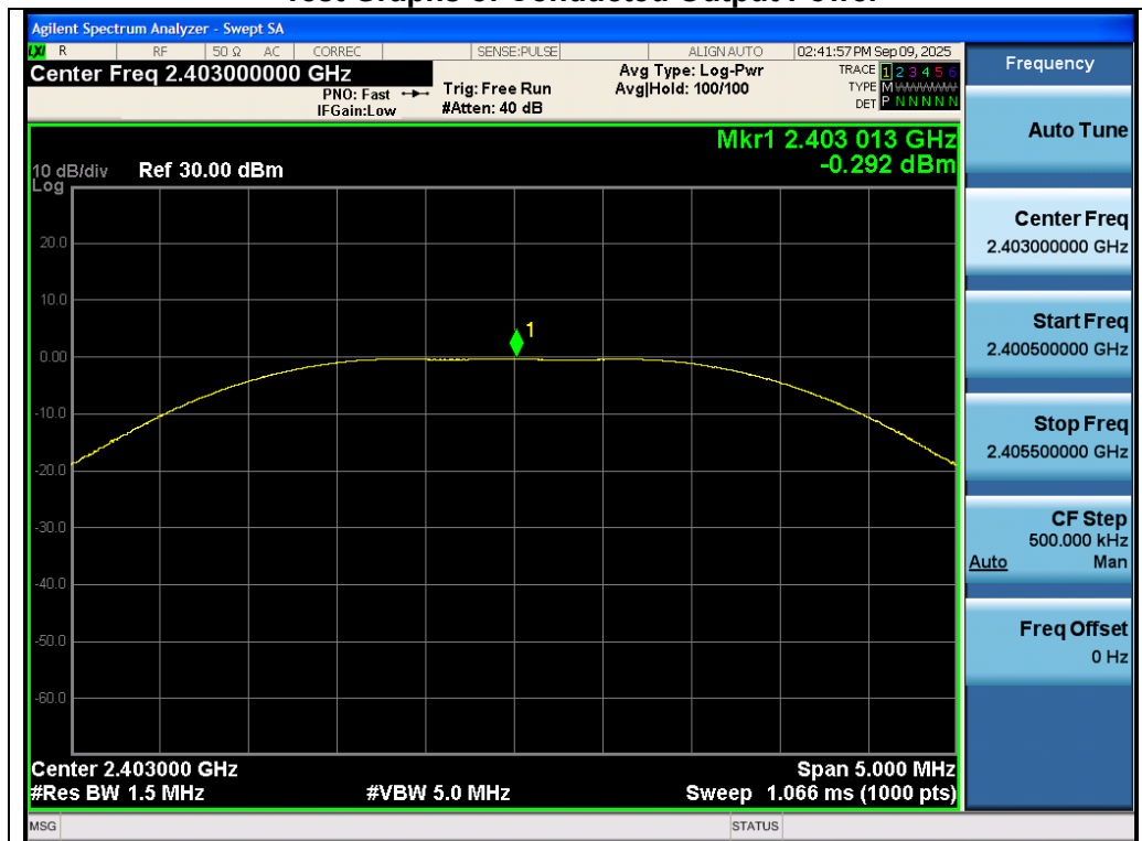
Test_Graph_SRD 2.4G_ANT1_2403_Peak Power
