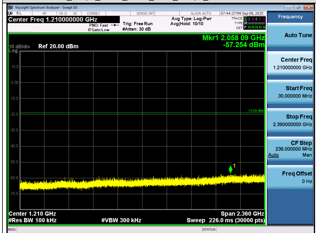
Test_Graph_LE2M_ANT1_2403_2Mbps_Lower Band Emissions
