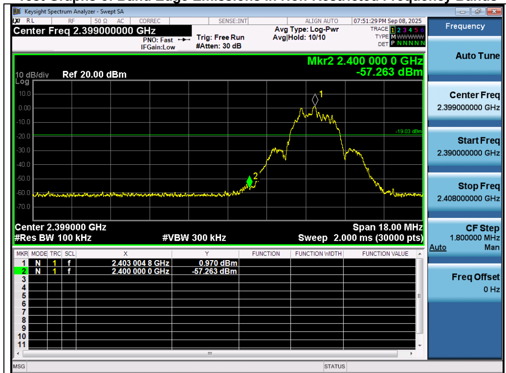
Test_Graph_LE2M_ANT1_2403_2Mbps_Lower Band Edge Emissions
