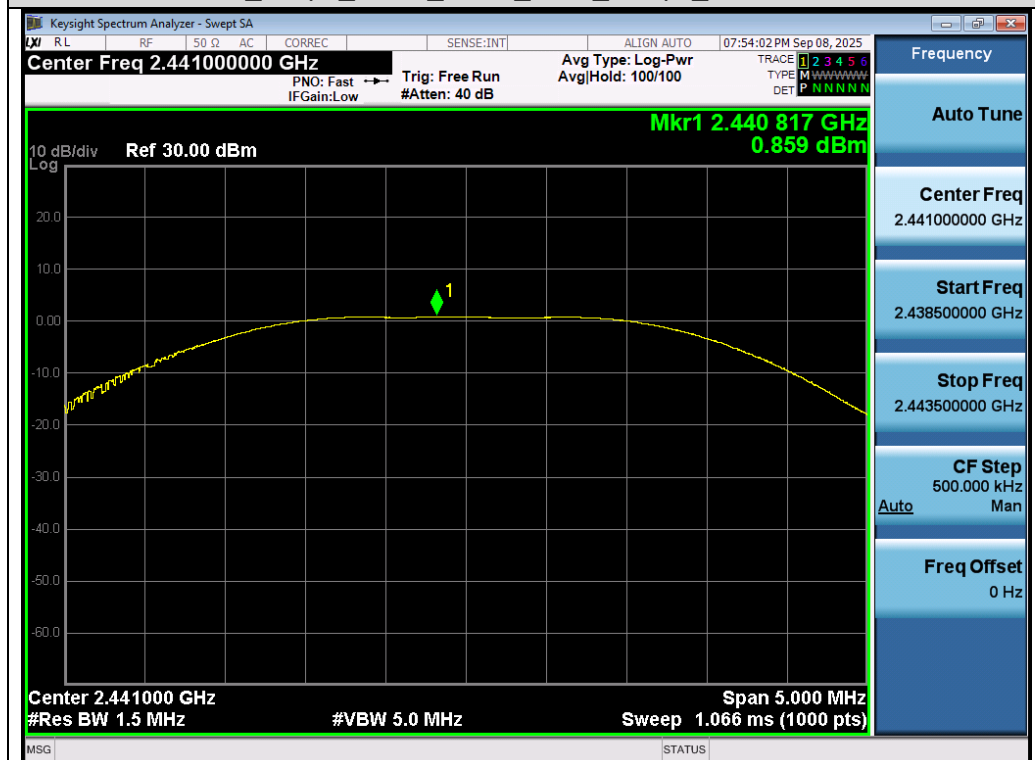
Test_Graph_LE2M_ANT1_2441_2Mbps_Peak Power
