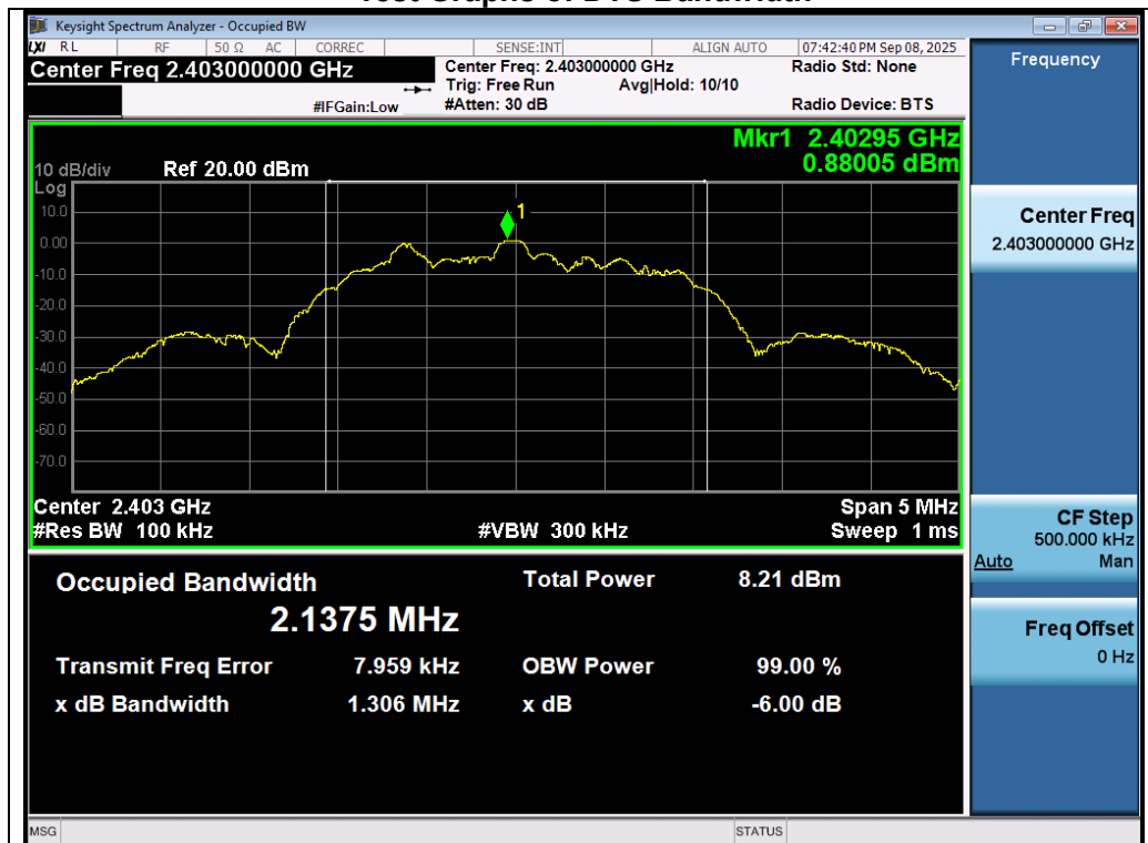
Test_Graph_LE2M_ANT1_2403_2Mbps_DTSBW
