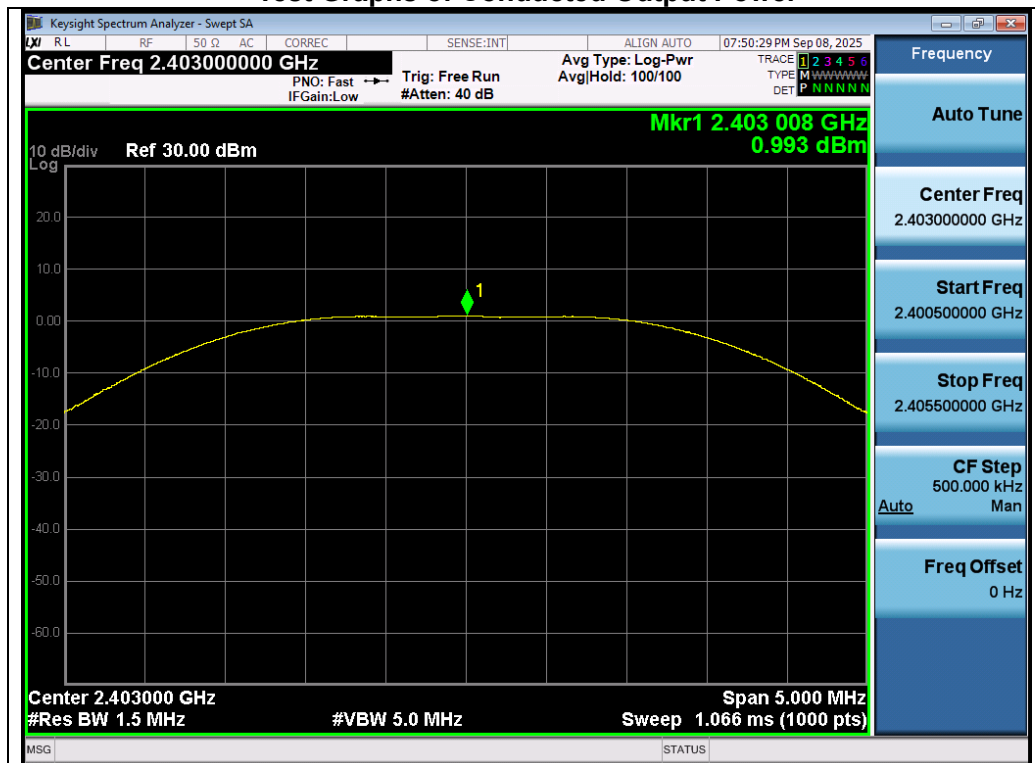
Test_Graph_LE2M_ANT1_2403_2Mbps_Peak Power
