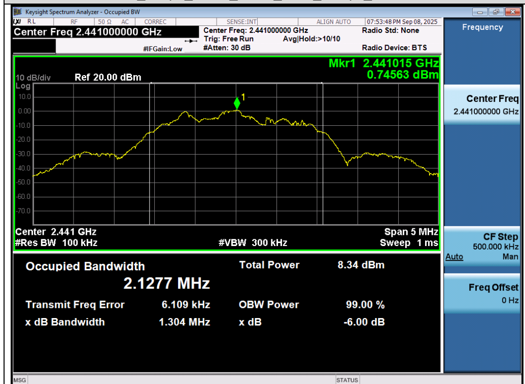
Test_Graph_LE2M_ANT1_2441_2Mbps_DTSBW
