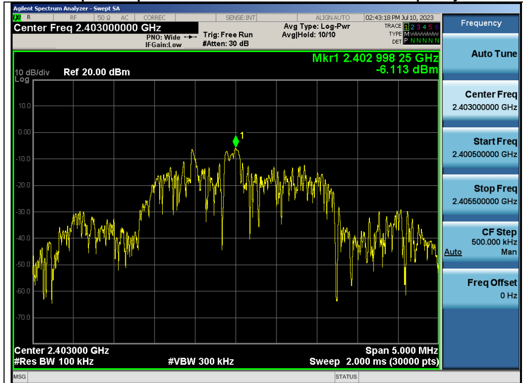
Test_Graph_ANT1_2403_Reference Level
