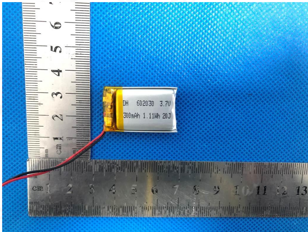
VIEW-2 OF BATTERY
