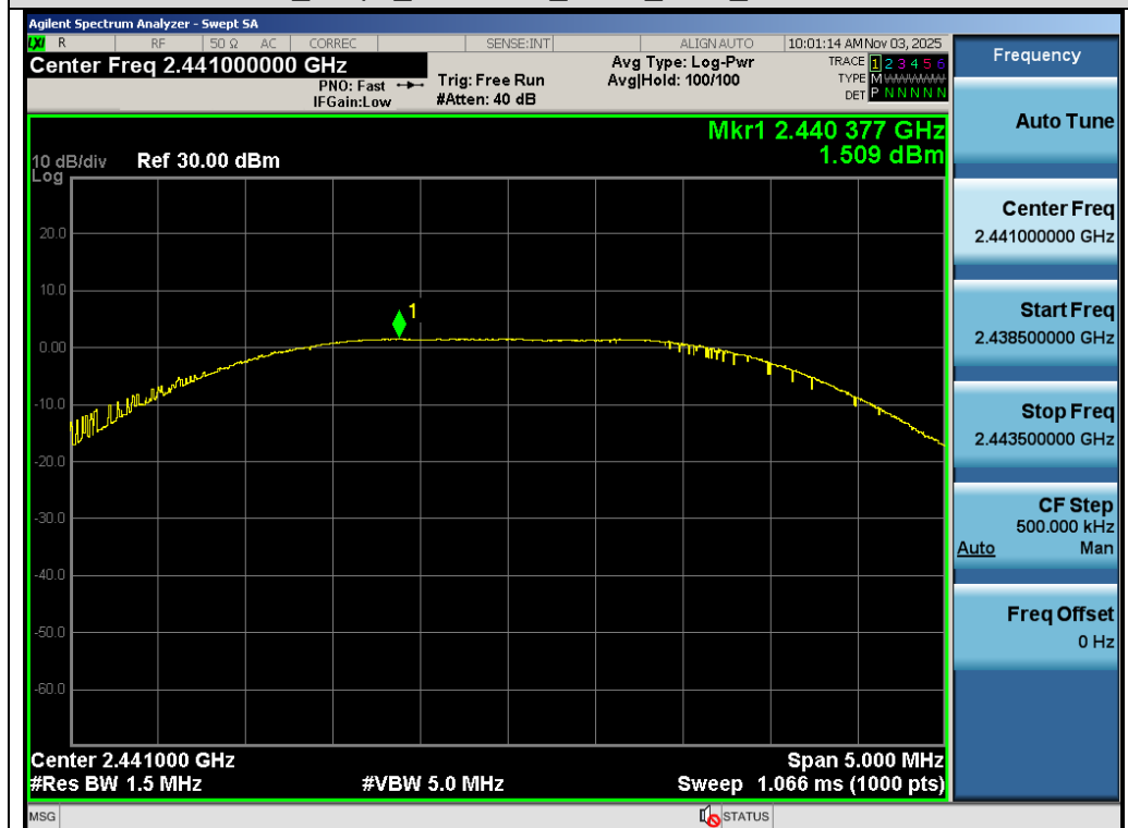
Test_Graph_SRD 2.4G_ANT1_2441_Peak Power
