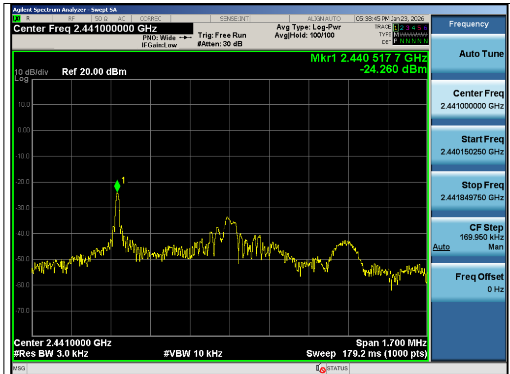
Test_Graph_2.4G_ANT1_2441_2Mbps_PSD
