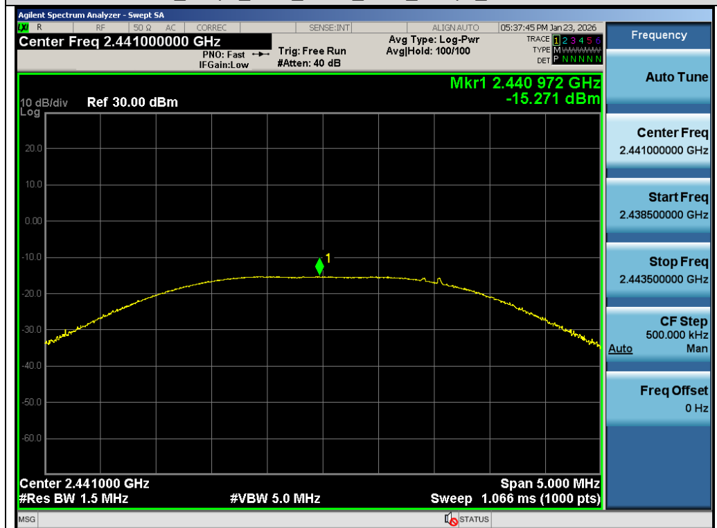
Test_Graph_2.4G_ANT1_2441_2Mbps_Peak Power
