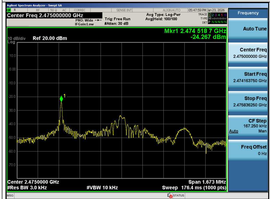
Test_Graph_2.4G_ANT1_2475_2Mbps_PSD
