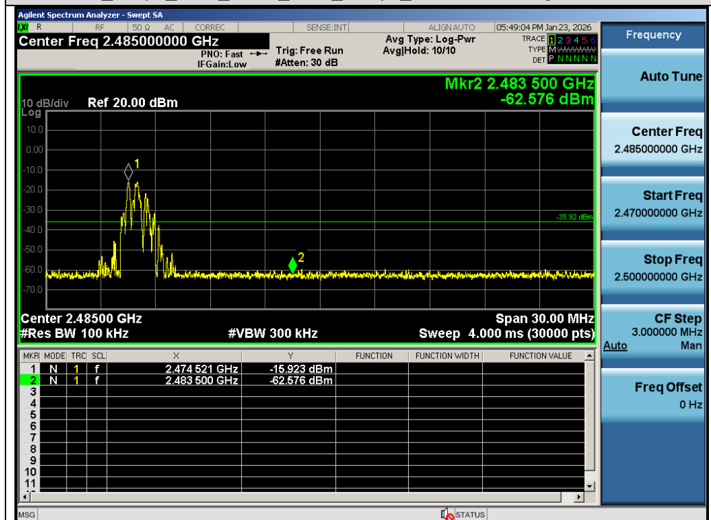
Test_Graph_2.4G_ANT1_2475_2Mbps_Higher Band Edge Emissions
