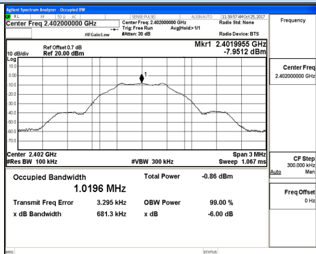
Channel 0 / 2402 MHz
