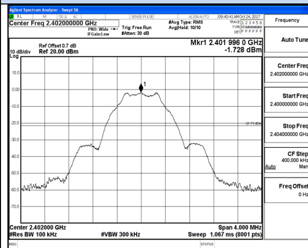
Channel 0 / 2402 MHz
