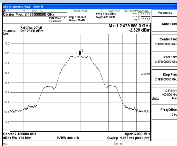
Channel 39 / 2480 MHz
