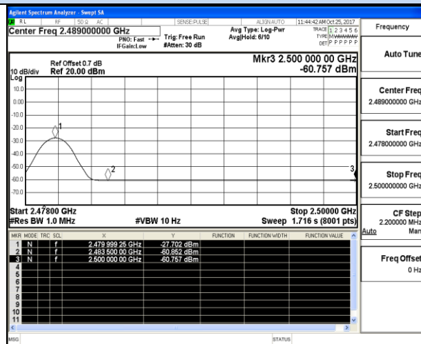
Channel 39 / 2480 MHz – Average
