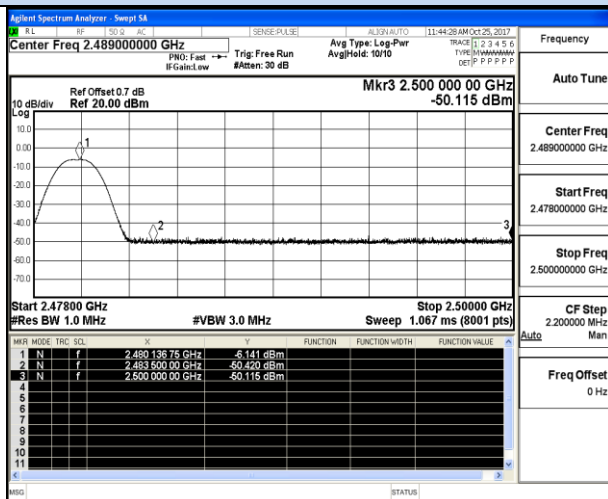
Channel 39 / 2480 MHz – Peak
