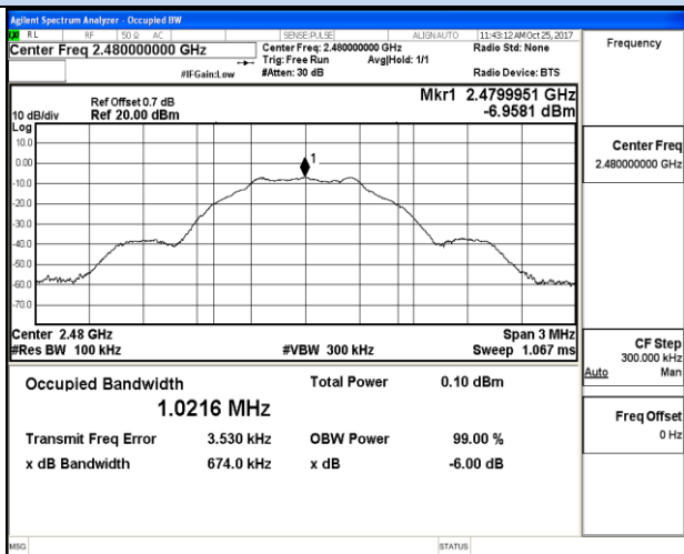
Channel 39 / 2480 MHz
