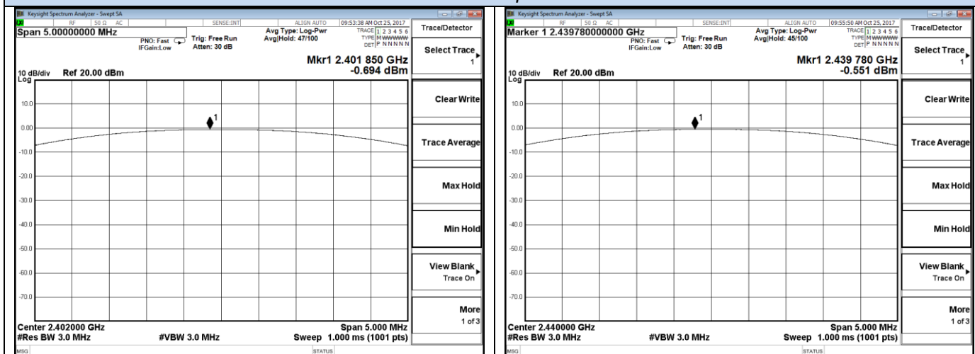
Channel 0 / 2402 MHz
