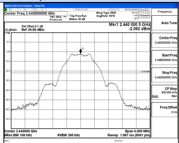
Channel 19 / 2440 MHz
