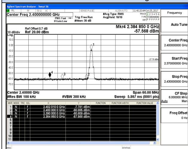
Channel 0 / 2402 MHz
