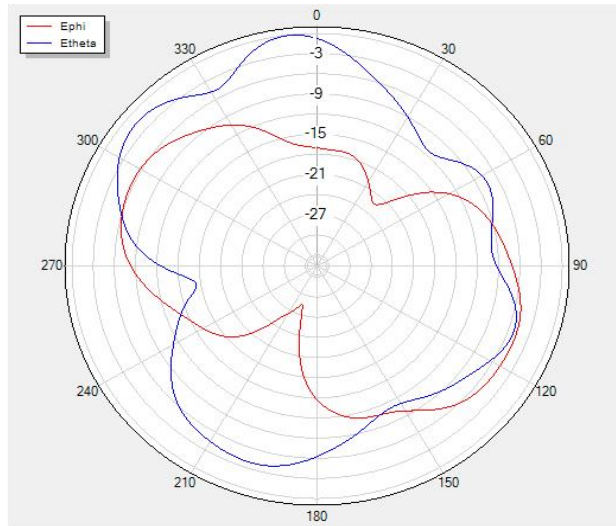
Theta=90 freq=2440MHz
