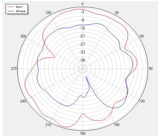
Phi=90 freq=2440MHz
