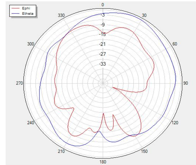
Phi=0 freq=2440MHz
