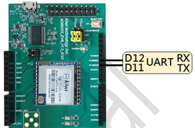
Figure 1-6 Pinout of ADB922
