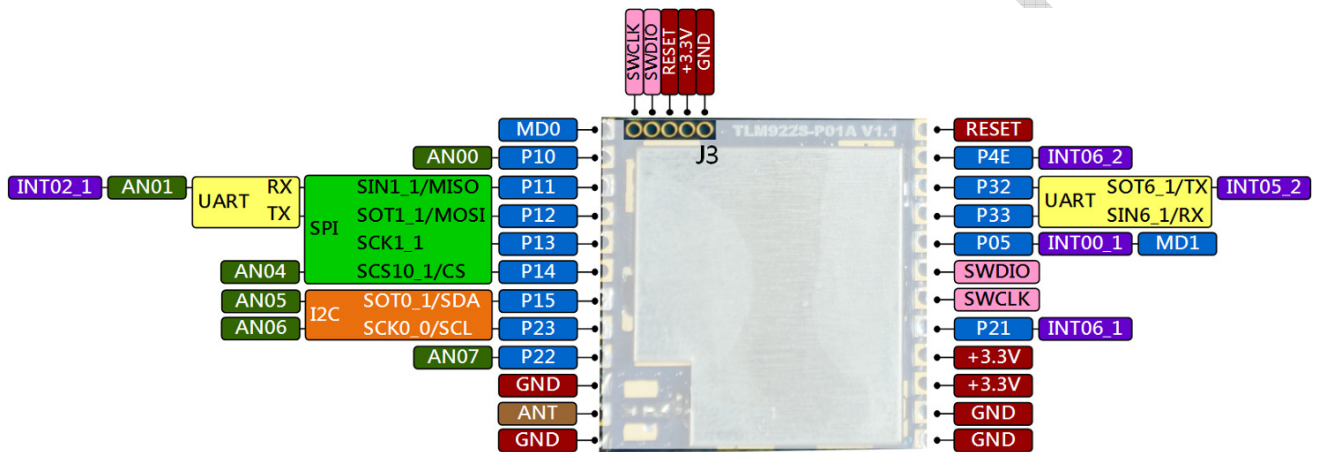
Figure 1-1 TLM922S-P01A Pinout
