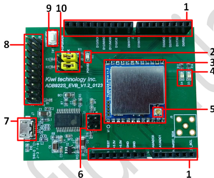
Figure 1-2 TLM922S-P01A EVB
