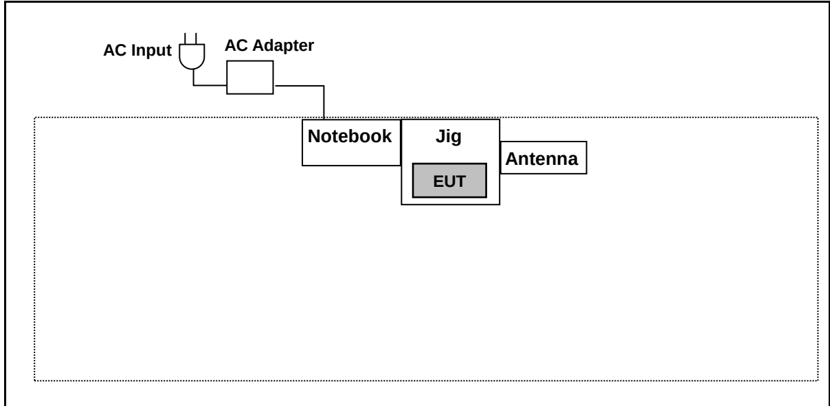
Radiated Emissions_Indoor
