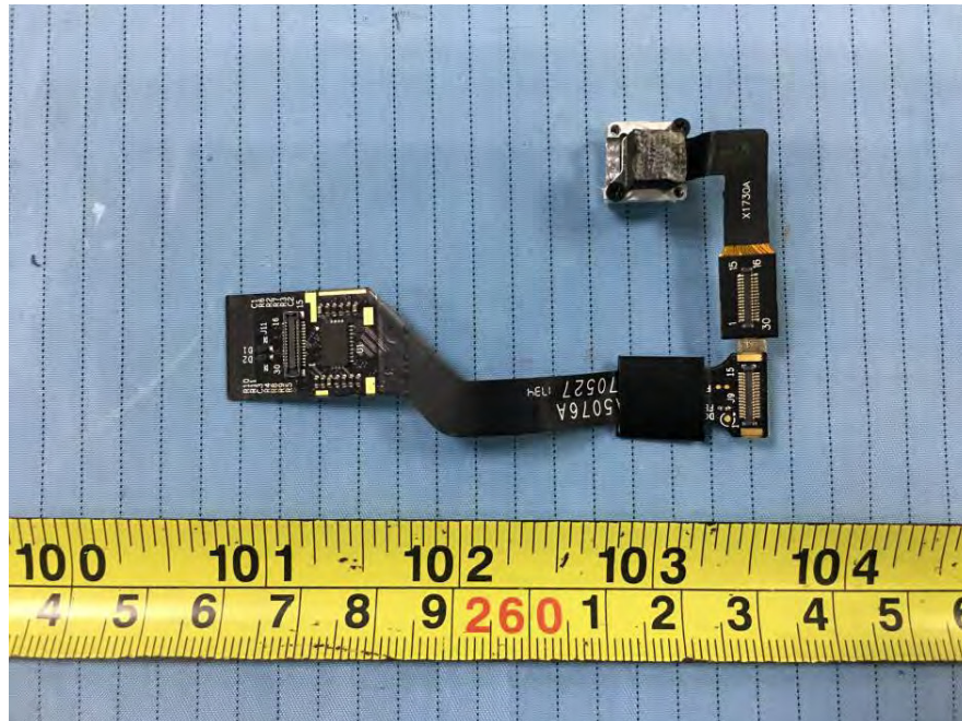
EUT –FPC connector View
