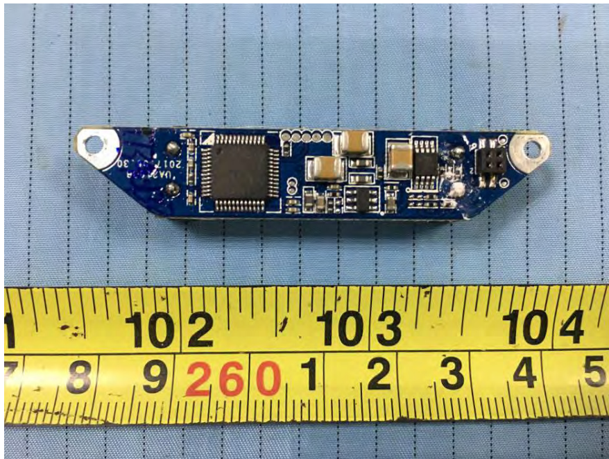
EUT –SONAR Board Bottom View
