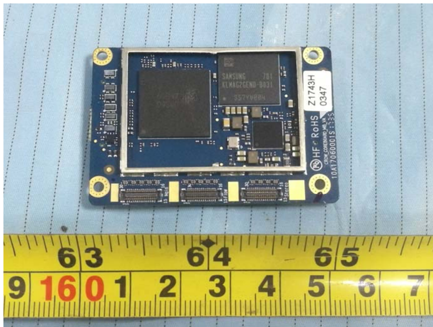
EUT – Main Board 12 Bottom Shielding off View
