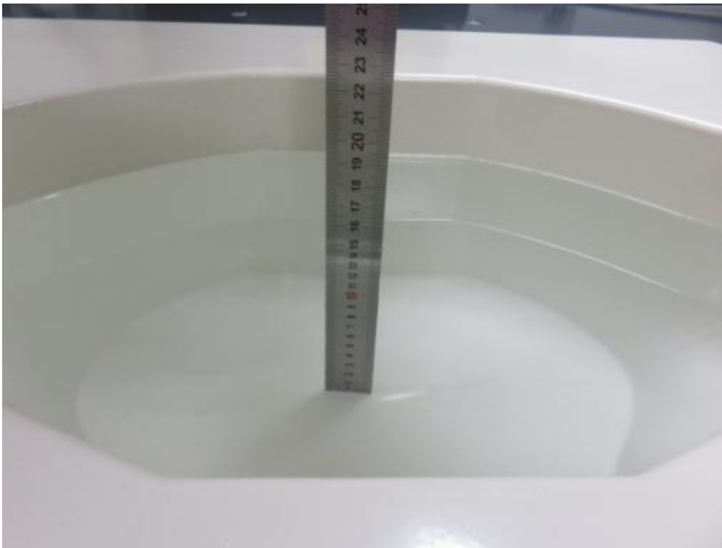
Photograph of the depth in the Body Phantom (5800MHz, 16.2cm depth)
