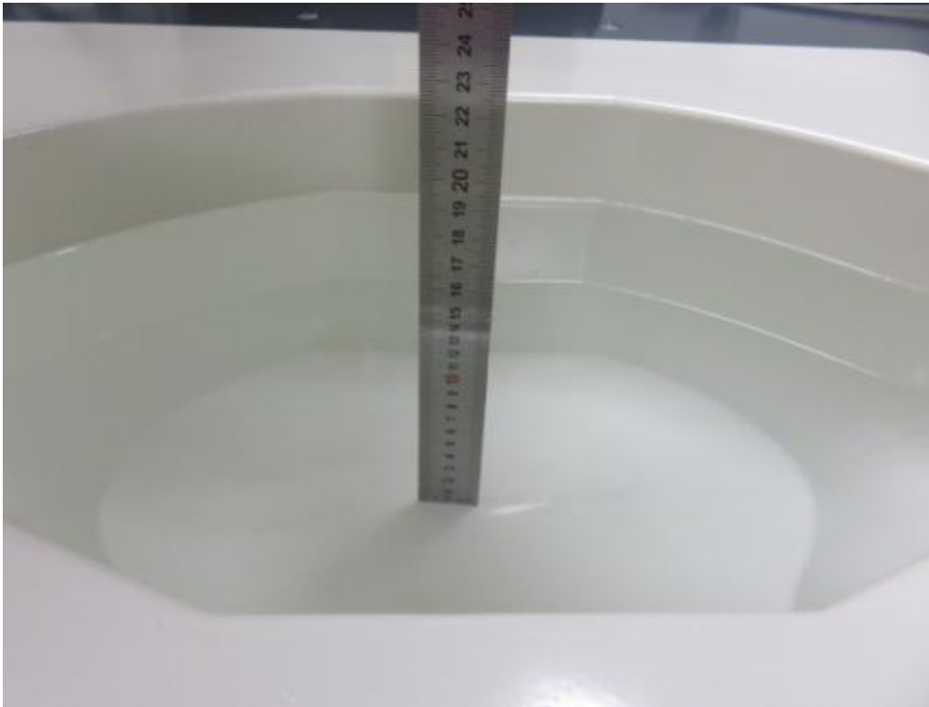
Photograph of the depth in the Body Phantom (5200MHz, 16.0cm depth)
