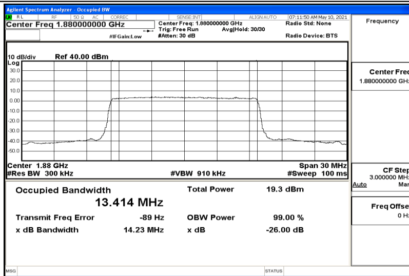
Band2-15MHz-QPSK-19125-75RB#0-13.432
