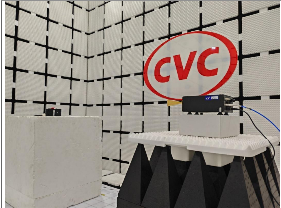
RADIATED EMISSION TEST (Above 40GHz)
