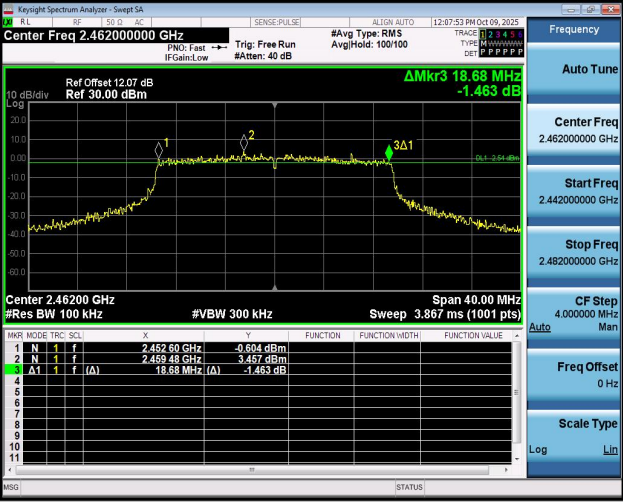
11AX20SISO-Ant1-2462-PASS
