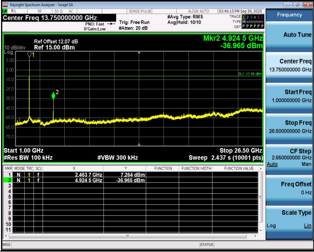
11B-Ant1-2462-1000~26500-PASS
