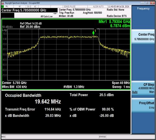
11AX20SISO-Ant1-5785
