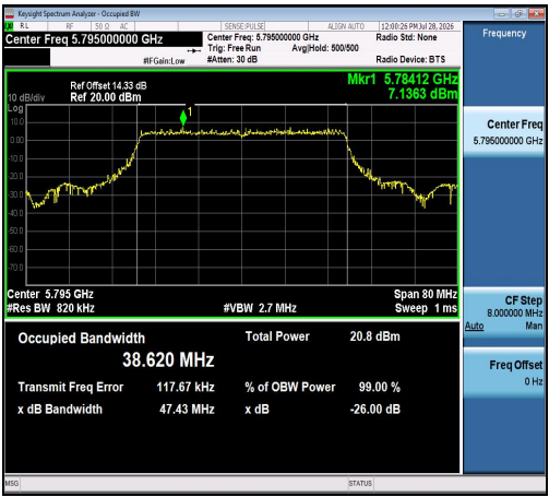
11AX40SISO-Ant1-5795
