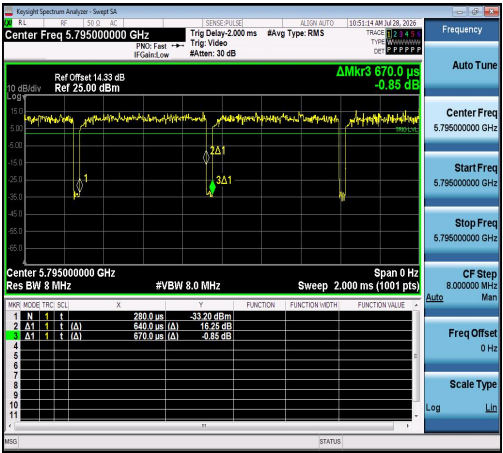
NTNV-11N40SISO-Ant1-5795
