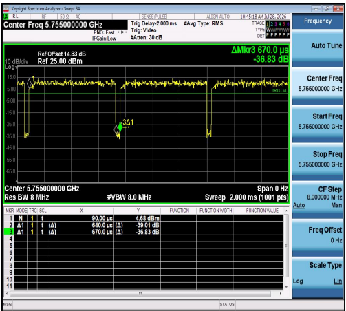
NTNV-11N40SISO-Ant1-5755
