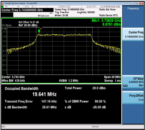
11AX20SISO-Ant1-5745
