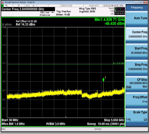
11N40SISO-Ant1-5795-30~5650-PASS
