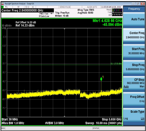
11AC20SISO-Ant1-5785-30~5650-PASS
