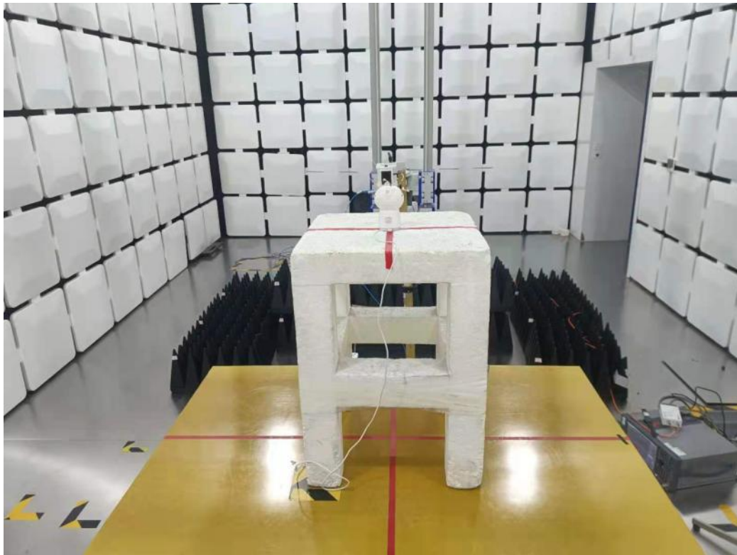
Radiated Spurious Emission Test (Above 18GHz)
