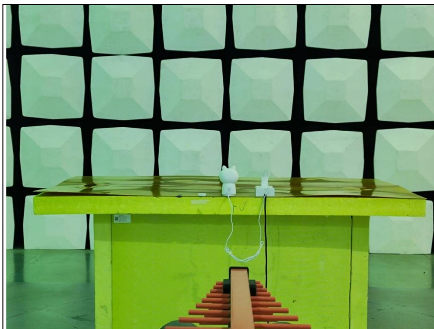
Radiated emissions at frequencies up to 1 GHz for FCC part 15B Mode 1& Mode 2
