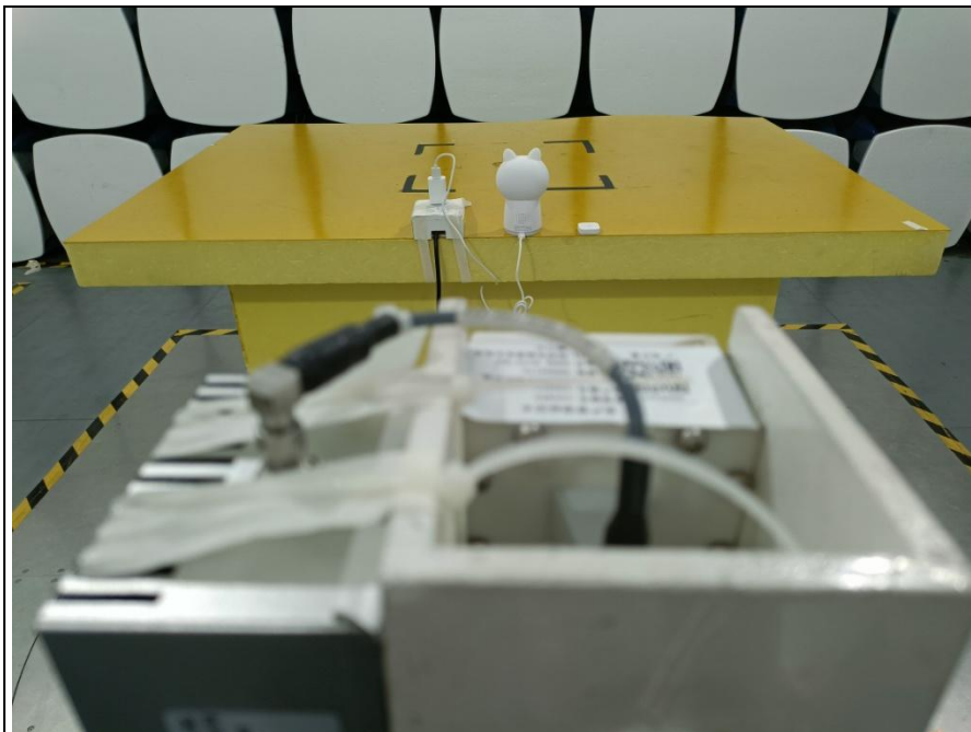
Radiated emissions at frequencies above 18GHz for FCC part 15B Mode 1& Mode 2
