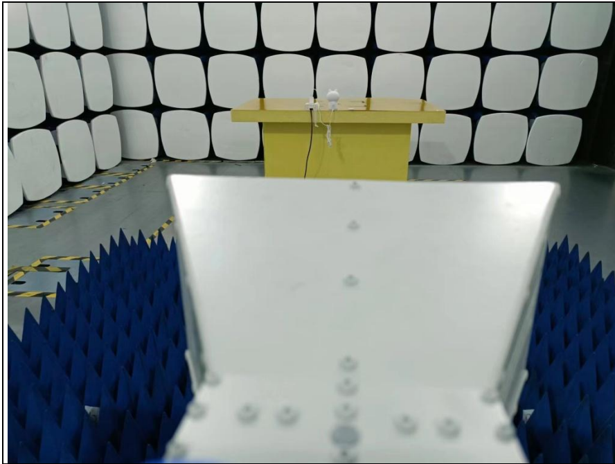
Radiated emissions at frequencies 1GHz to 18GHz for FCC part 15B Mode 1& Mode 2
