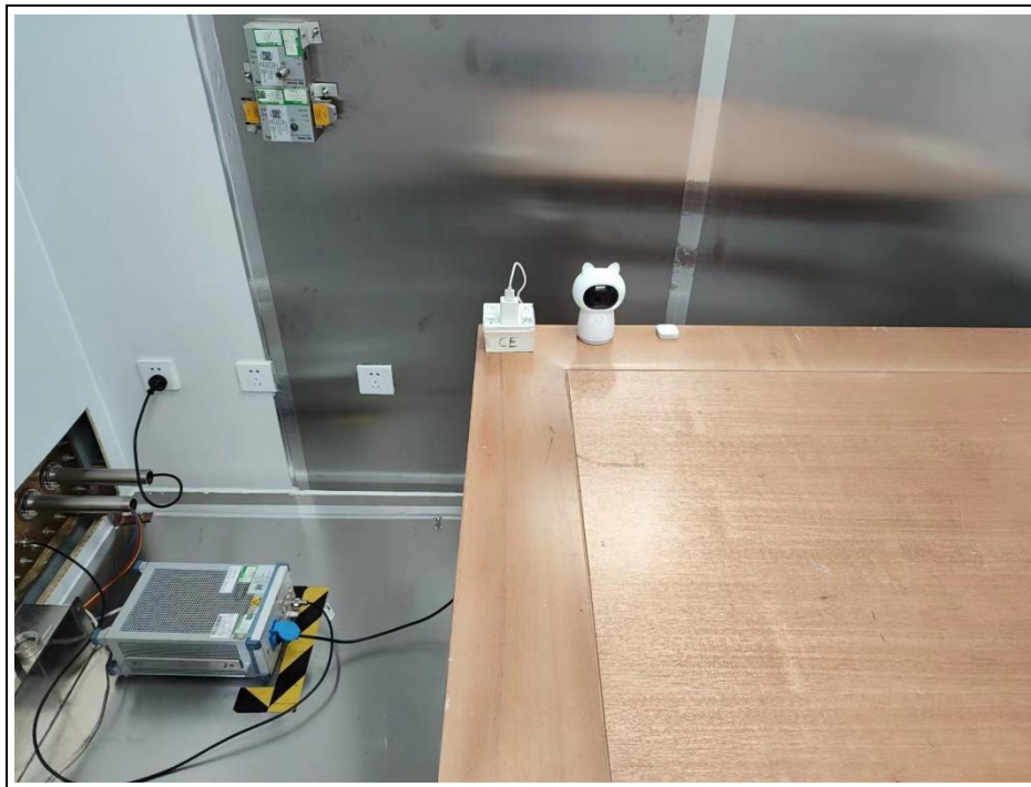
conducted emissions for FCC part 15B Mode 1& Mode 2
