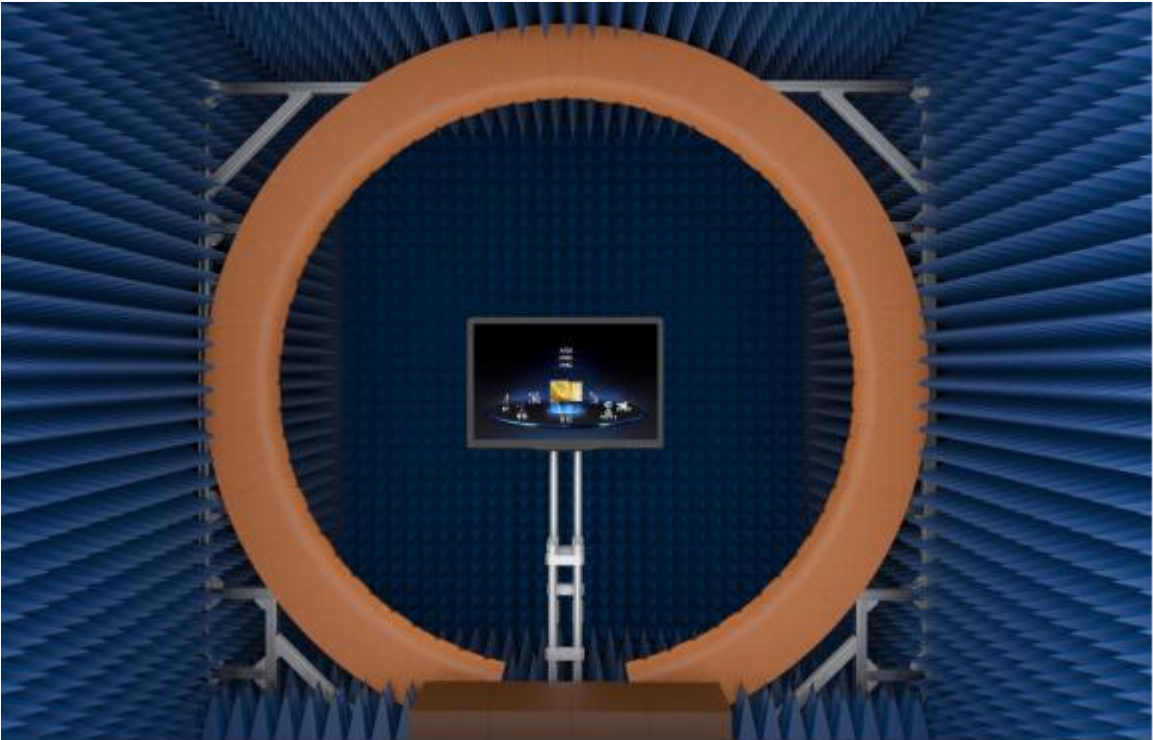
The industry's top 64 sensors OTA chamber
