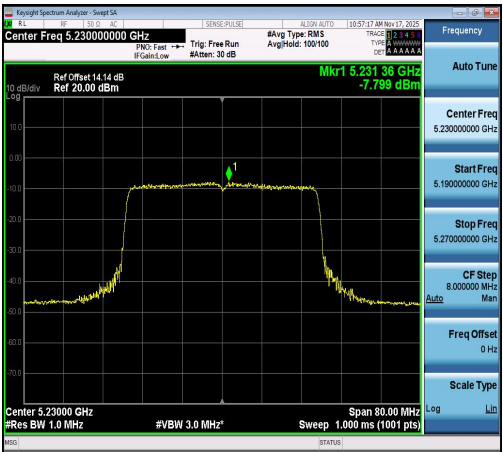
11AX40SISO-Ant1-5230-PASS
