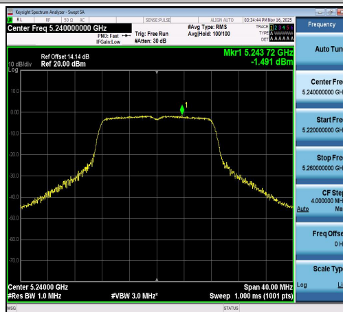
11A-Ant1-5240-PASS
