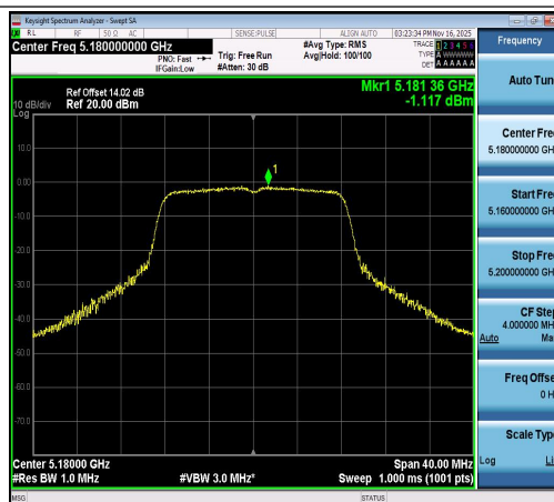
11A-Ant1-5180-PASS
