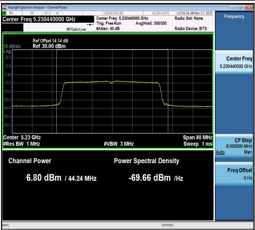
11AX40ISO-Ant1-5230-PASS
