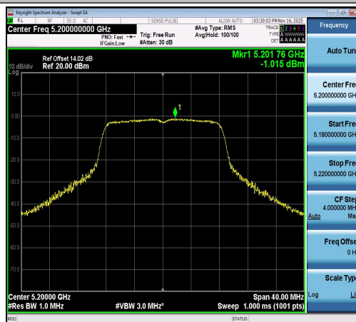
11A-Ant1-5200-PASS
