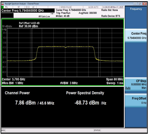
11AX40ISO-Ant1-5795-PASS
