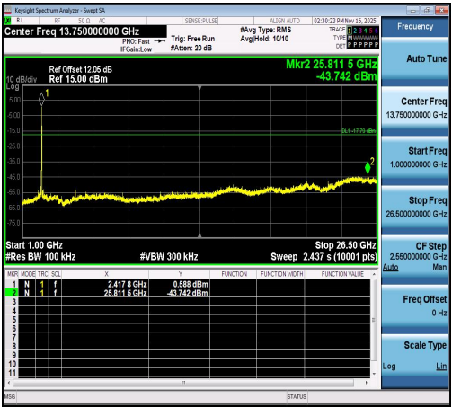
11AX20SISO-Ant1-2412-1000~26500-PASS
