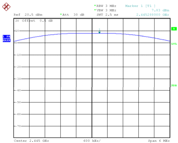
Mode: TX QPSK channel 8
