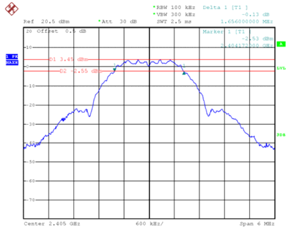
Mode: TX QPSK channel 0
