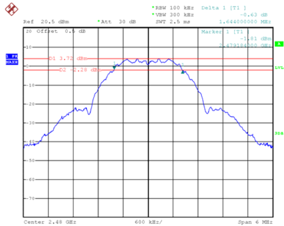
Mode: TX QPSK channel 15
