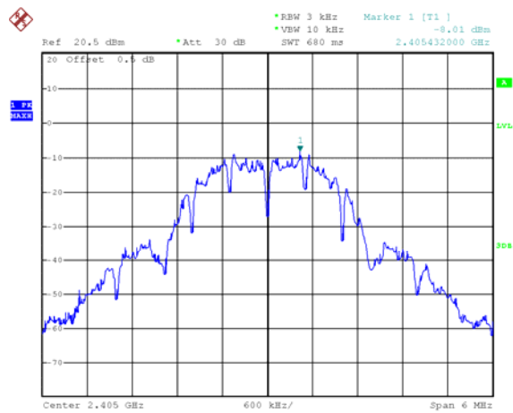
Mode: TX QPSK channel 0
