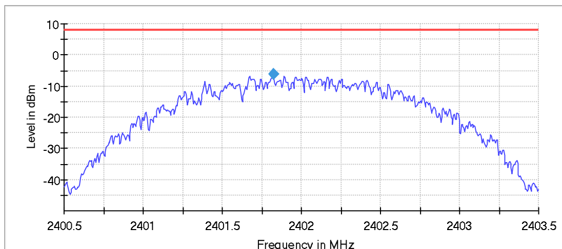
Data of BLE 2M Peak Power Spectral Density
