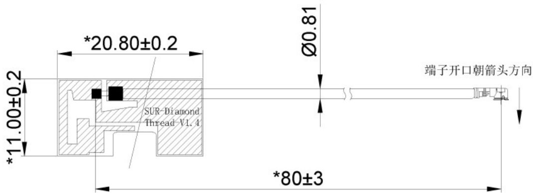
BLE& Thread Antenna
