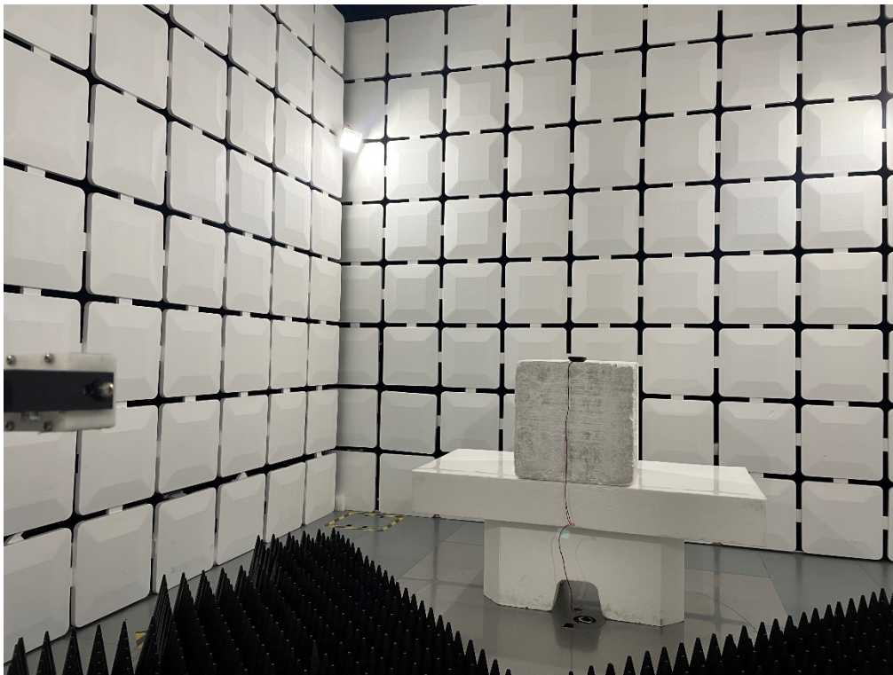
Description: Radiated Emission Test Setup for Above 18-40GHz
